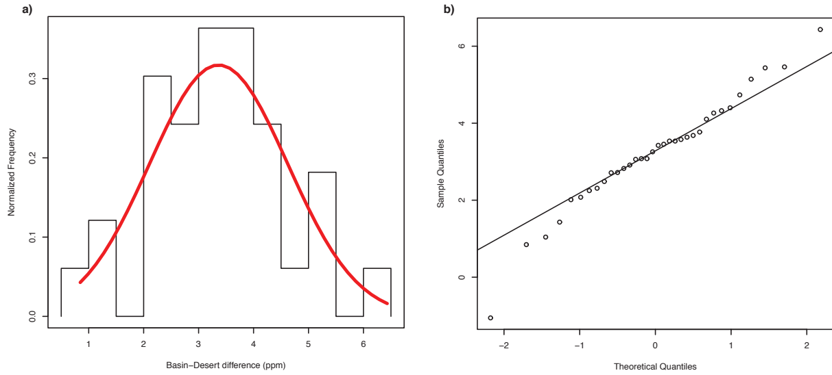
Figure S3: Distribution of Los Angeles basin-desert difference. a) Histogram of basin-desert difference for the GOSAT XCO2 observations in Los Angeles. The red line represents a Gaussian distribution. b) Quantile-quantile plot of 10-day average basin-desert differences in LA. The solid line represents a Gaussian distribution.
