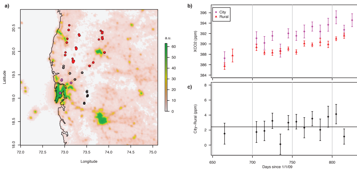
Figure S4: Observed X_{CO_2} urban dome of Mumbai. a) Nightlights map of Mumbai megacity and surroundings. Selected GOSAT observations over the city (pink circles) and nearby rural areas (red triangles). b) Time-series for city and rural observations averaged in 10-day bins. c) The difference between 10-day block averages of city and rural observations. The solid black line shows the average difference ( 2.4 \pm 1.2 ppm).
