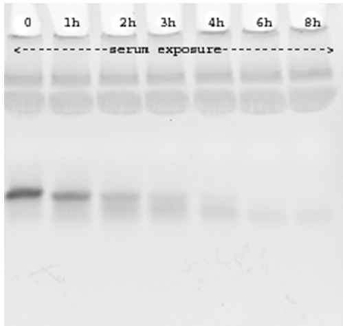
Supplementary Figure 3 Degradation kinetics of synthetic siRNA in mouse serum. 40 pmol siCNTL was incubated in 20 \mu L mouse serum (active) at 37 ^{\circ} C for indicated times before being electrophoresed on a 15% (wt/vol) TBE gel.
