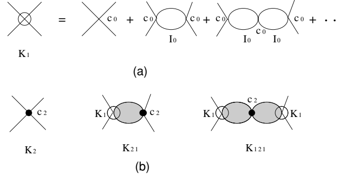
FIG. 1. Diagrammatic representation of K_1 , K_2 , K_{21} , and K_{121} . Panel (a) depicts K_1 as a sum of the iterations of c_0 , Eq. (27), with a crossing point as c_0 . The open bubble is the regulated Green's function I_0 . Panel (b) shows K_2 , K_{21} , and K_{121} as in Eqs. (29), with an open circled vertex as K_1 and with a dot vertex as c_2 . The shaded bubble is a regulated Green's function weighted with vertex momenta, I_2 .
