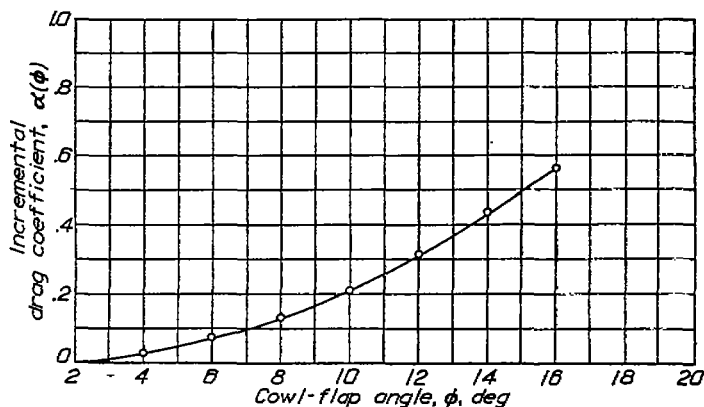
FIGURE 4.—Incremental drag coefficient for various cowl-flap angles.
