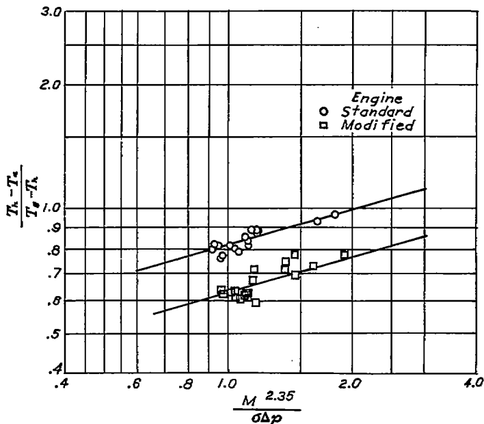
FIGURE 7.—Comparison between correlation of cooling data for standard and modified engines in port inboard nacelles of airplane, based on temperature of hottest rear-row exhaust-valve seat.
