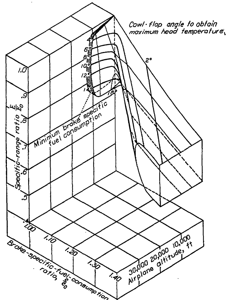
FIGURE 12.—Effect of airplane altitude and brake specific fuel consumption on specific range with cowl flaps set for proper engine cooling. Standard-engine installation; indicated-air-speed ratio, 1.00; airplane weight, 100,000 pounds.
