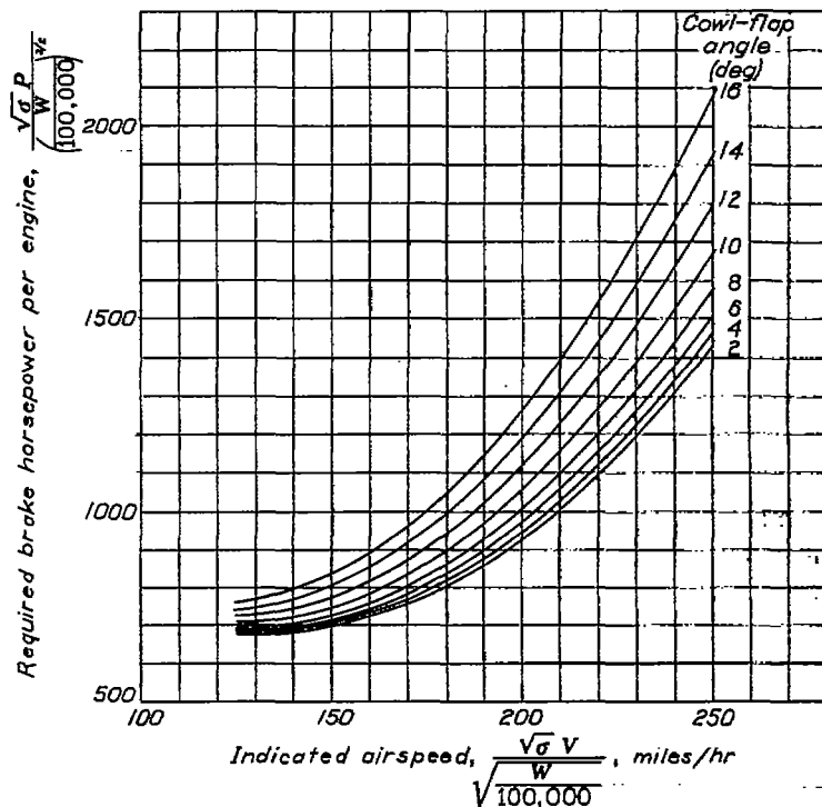
FIGURE 5.—Approximate power required by four-engine heavy bomber for level-flight cruising.
