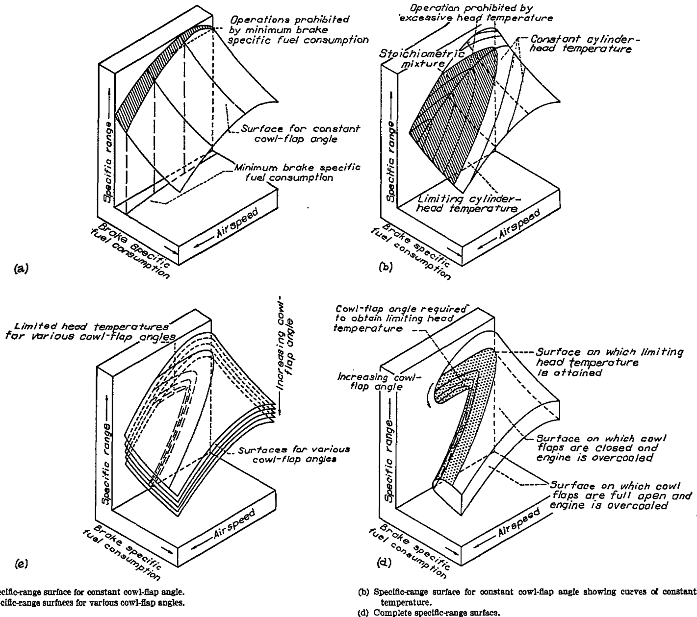
FIGURE 10.—Development of surfaces showing specific range with proper engine cooling as function of flight and engine variables.
