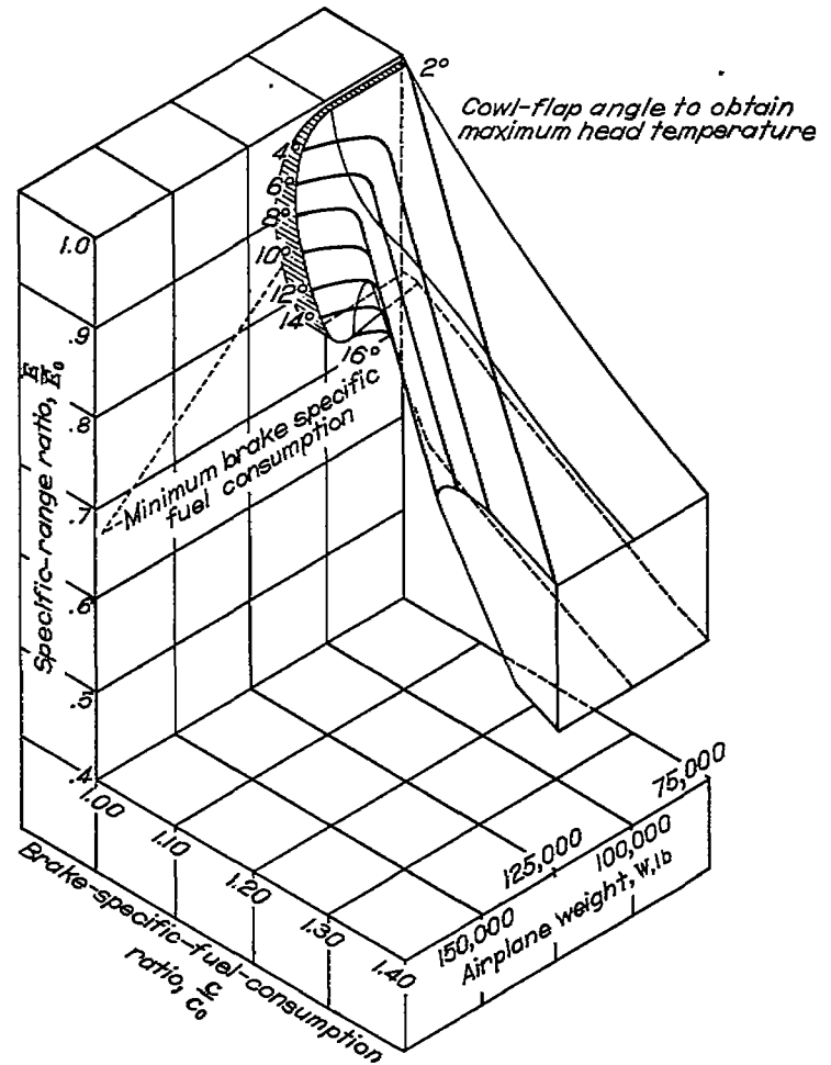
FIGURE 13.—Effect of airplane weight and brake specific fuel consumption on specific range with cowl flaps set for proper engine cooling. Standard-engine installation; indicated-air-speed ratio, 1.00; altitude, 5000 feet.
