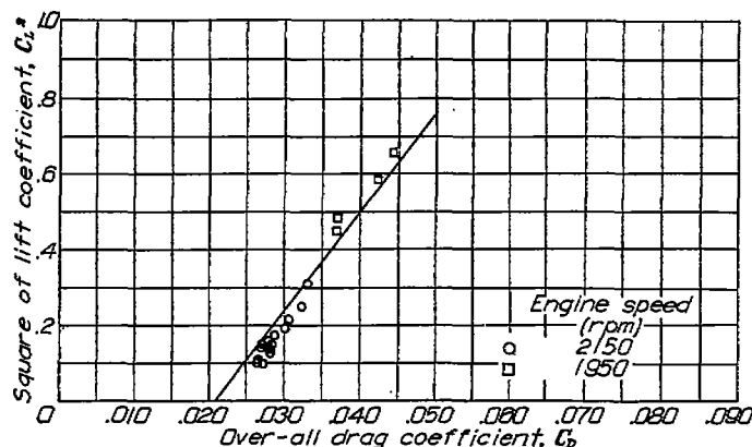
FIGURE 3.—Relation between square of lift coefficient and drag coefficient. Cowl flaps at 2° (closed) position; propulsive efficiency, 0.85.
