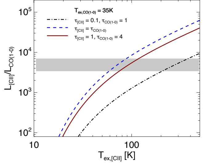
Figure 11. The L_{\text{[CII]}}/L_{\text{CO}(1-0)} ratio as a function of the [CII] excitation temperature for a fixed T_{\text{ex,CO}(1-0)} = 35 K. The observed L_{\text{[CII]}}/L_{\text{CO}(1-0)} ratio in the SPT DSFG sources (grey shaded area) is achieved within T_{\text{ex,[CII]}} \sim 60 - 90 K for equal [CII] and CO optical depth (blue curve). In the case of \tau_{\text{[CII]}} = 1 and \tau_{\text{CO}(1-0)} = 4 , the L_{\text{[CII]}}/L_{\text{CO}(1-0)} ratio is achieved for T_{\text{ex,[CII]}} = 85 - 110 K. The optically thin \tau_{\text{[CII]}} = 0.1 and nearly optically thick \tau_{\text{CO}(1-0)} = 1 case is reached by [CII] excitation temperatures in the range \sim 240 - 330 K (black dashed curve).
