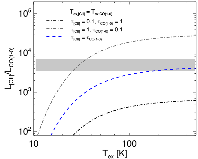
Figure 9. The L_{\text{[CII]}}/L_{\text{CO}(1-0)} ratio predicted from the source functions versus equal [CII] and CO(1-0) excitation temperatures ( T_{\text{ex,[CII]}} = T_{\text{ex,CO}(1-0)} ), for three different cases of the optical depth: i ) optically thin [CII] and optically thick CO(1-0) (the black dot-dashed curve), ii ) optically thick [CII] and optically thin CO(1-0) - (the grey dot-dashed curve), iii ) same optical depth of [CII] and CO(1-0) (blue dashed curve). The grey shaded area represents the 1\sigma spread of the L_{\text{[CII]}}/L_{\text{CO}(1-0)} ratio in the SPT sample. Case i underpredicts the ratio by an order of magnitude. Cases ii and iii can both reproduce the observed ratio. However, we know from ^{12}\text{CO} to ^{13}\text{CO} ratios that CO is optically thick (e.g. Spilker et al. 2014), which rules out case ii . Only case iii , implying optically thick CO and [CII], is consistent with all observational data.
