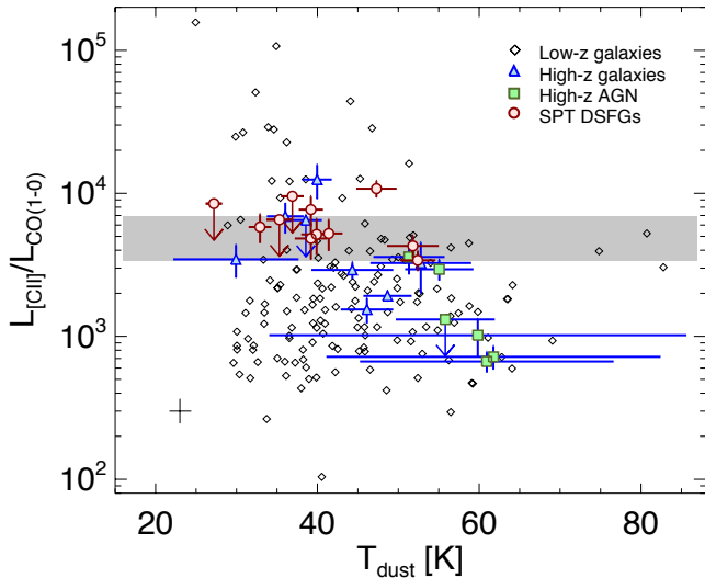
Figure 8. L_{[CII]}/L_{CO(1-0)} vs T_d for the SPT sources and the low and high- z comparison sample. The typical error bar is represented by the black cross. The grey shaded area represents the 1\sigma spread of the L_{[CII]}/L_{CO(1-0)} ratio in the SPT sample. Both the SPT sources and the low- z sample do not show any dependence on T_d . The high- z AGN-dominated sources are both warmer and have fainter [CII] relative to CO.
