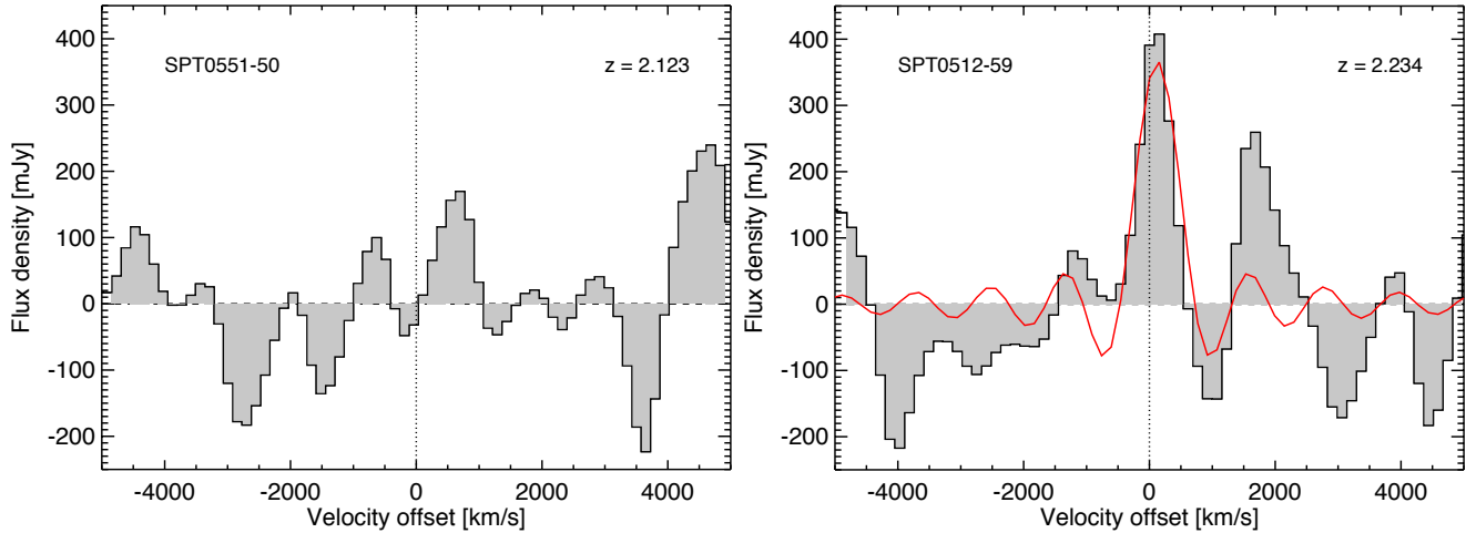
Figure 2. Herschel SPIRE FTS spectra for SPT0551-50 and SPT0512-59. Left: Non-detection of the [CII] emission line for SPT0551-50. Right: Detection of [CII] emission line for SPT0512-59. The continuous red curve is the sinc-function used to fit the [CII] line (see Valtchanov et al. 2011).
