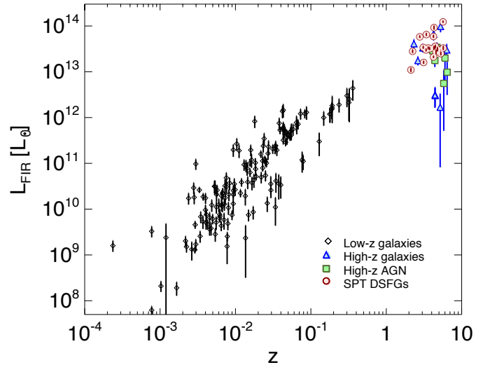
Figure 3. Observed L_{FIR} vs redshift for the 20 SPT sources and the comparison sample. No L_{FIR} have been corrected for lensing magnification factors. The distribution shows the Malmquist bias where high- z galaxies require either lensing magnification or very high intrinsic FIR luminosity of L_{FIR} \gtrsim 10^{12} L_{\odot} to be included in the parent sample. The evolution of the luminosity function and the smaller comoving volume at low redshifts imply that objects with similar high intrinsic L_{FIR} are missing from the low- z sample. However, the most highly lensed DSFGs may have similar intrinsic L_{FIR} than the most luminous sources in the local sample.
