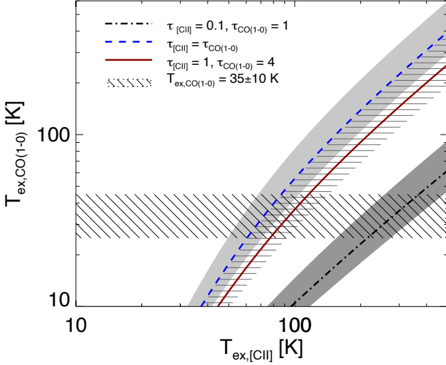
Figure 10. T_{\text{ex,CO}(1-0)} as a function of T_{\text{ex,[CII]}} . In all cases, the excitation temperature of [CII] is higher than for CO(1-0). The blue dashed curve with the light grey shaded area shows the observed L_{\text{[CII]}}/L_{\text{CO}(1-0)} range of SPT DSFGs in the case of equal [CII] and CO optical depths. The red continuous curve and hashed area illustrates that the difference between the excitation temperatures becomes even more significant for \tau_{\text{[CII]}}=1 and \tau_{\text{CO}(1-0)}=4 . The dot-dashed curve and the dark grey shaded area illustrate the case of \tau_{\text{[CII]}}=0.1 and \tau_{\text{CO}(1-0)}=1 . The hatched horizontal area marks T_{\text{ex,CO}(1-0)} = 35 \pm 10 K.
