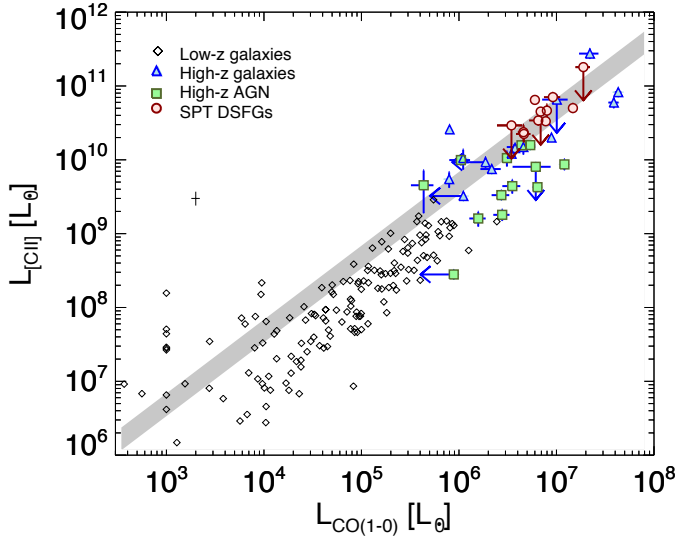
Figure 7. The [CII] luminosity versus the CO luminosity for the SPT DSFGs and the comparison low and high- z samples. These star forming systems show a correlation between the [CII] and CO(1-0) luminosities. Fitting a ratio to 11 SPT sources with [CII] detections and CO(1-0) data yields a slope of \sim 5200 . The width of the grey shaded area represents a 1\sigma spread, \sim 5200 \pm 1800 . Fitting a ratio to the low- z sample yields a slope of 1300 \pm 440 . The typical error bar for the low- z sources is represented by the black cross.
