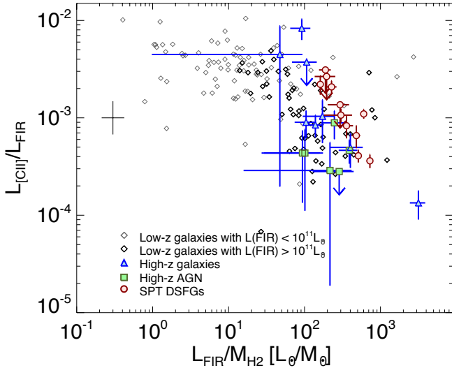
Figure 5. L_{[CII]}/L_{FIR} vs the FIR luminosity normalised by the molecular gas mass. The molecular gas mass is derived assuming a conversion factor of \alpha_{CO} = 0.8 M_{\odot} (\text{K km s}^{-1} \text{pc}^{-2})^{-1} . The L_{FIR}/M_{H_2} ratio is expected to be proportional to the number of stars formed in a galaxy per unit molecular gas mass (Graciá-Carpio et al. 2011). This M_{H_2} normalisation removes the uncertainty due to the unknown lensing magnification factors, and reduces the scatter seen in Figure 4, but the deficit in the L_{[CII]}/L_{FIR} ratio still persists. The typical error bar is represented by the black cross.
