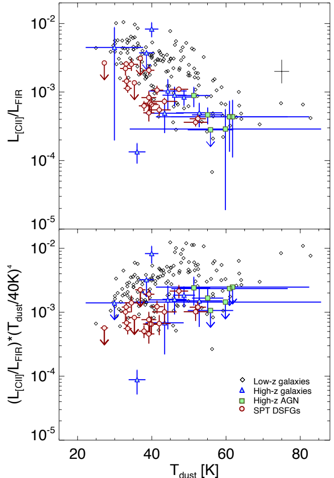
Figure 6. Top panel: L_{[CII]}/L_{FIR} vs T_d for the SPT DSFGs and the low and high- z comparison sample. The anti-correlation between the L_{[CII]}/L_{FIR} ratios and the dust temperatures is seen for both low- and high- z sources, and is expected because the Stefan-Boltzmann law predicts L_{FIR} \propto T_d^4 . Bottom panel: [CII] \times T_d^4 / L_{FIR} vs T_d for the SPT DSFGs and the low and high- z comparison sample. Multiplying the L_{[CII]}/L_{FIR} ratio with T_d^4 cancels out the temperature dependence of the Stefan-Boltzmann law. All lensing magnification factors and beam filling factors cancel in both panels, and the typical error bar is represented by the black cross.
