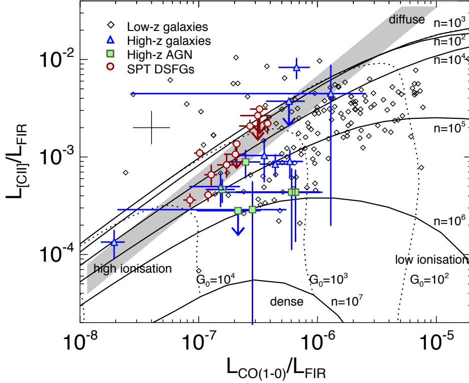
Figure 12. L_{[\text{CII}]} / L_{\text{FIR}} vs L_{\text{CO}(1-0)} / L_{\text{FIR}} for the SPT sources and the low and high- z comparison sample. The figure (e.g. Wolfire et al. 1989; Stacey et al. 2010) compares the values of the strength of the radiation field G_0 and the density n for low and high- z sources. The diagram is independent of lensing magnification factors for high- z source and beam filling factors for low- z sources as both the [\text{CII}] and \text{CO}(1-0) emission is normalised by the FIR luminosity. The typical error bar is represented by the black cross. To compare the observations with the model contours Stacey et al. (2010) assume that 70% of the [\text{CII}] emission originate from PDRs. The grey shaded area represents the 1\sigma spread of the L_{[\text{CII}]} / L_{\text{CO}(1-0)} ratio in the SPT sample.
