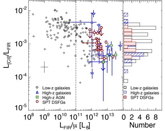
Figure 4. L_{\text{[CII]}}/L_{\text{FIR}} vs L_{\text{FIR}} for SPT sources and the comparison sample. As reported in previous versions of this plot, the L_{\text{[CII]}}/L_{\text{FIR}} is anti-correlated with L_{\text{FIR}} . In particular at L \gtrsim 10^{11} L_{\odot} , the L_{\text{[CII]}}/L_{\text{FIR}} ratio drops and has a larger spread. For the SPT sources without known lensing models, we assume a lensing magnification factor of 14.1 (and an uncertainty which encompasses the range of 5 to 22 from the known models). The typical error bar for the literature sources is represented by the black cross in the lower left. The histogram on the right shows the distribution of galaxies with L_{\text{FIR}} \gtrsim 10^{11} L_{\odot} .
