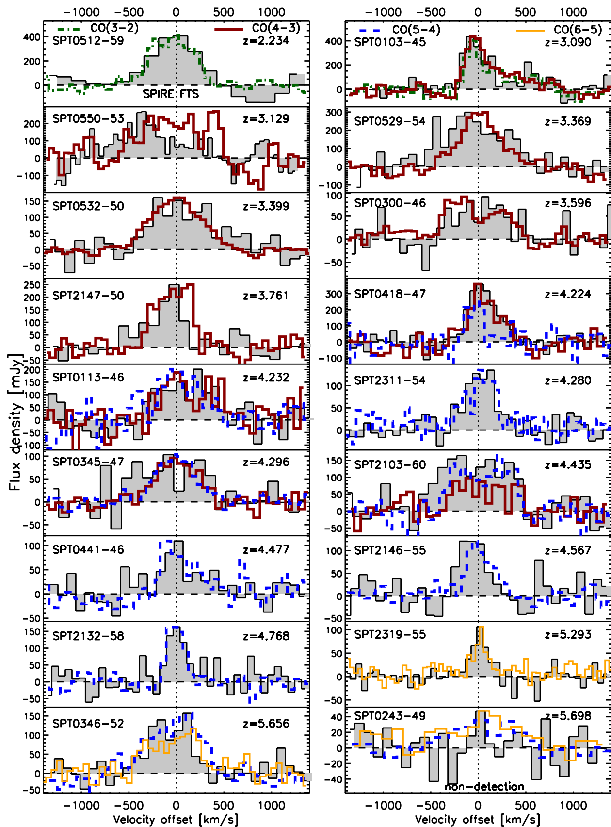
Figure 1. Comparison of the velocity profiles of the [\text{CII}] lines detected with APEX/FLASH and SPIRE FTS (grey filled profiles) and mid- J CO line observed with ALMA in Cycle 0 (coloured lines; Weiß et al. 2013). The CO lines have been scaled to match the [\text{CII}] peak flux. The similarities between the CO and [\text{CII}] lines for individual sources suggest that the spatial distributions are similar and differential lensing is not significant.
