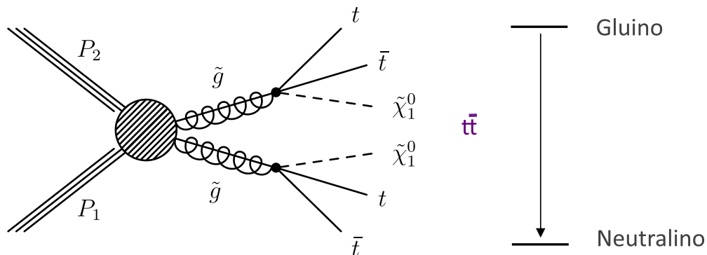
FIG. 10 (color online). Event diagram and a schematic superpartner mass spectrum for the SMS T1ttt scenario.
