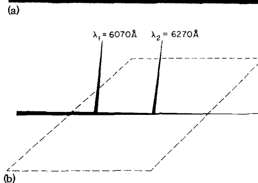
FIG. 2. (a) Double-exposure photograph showing the reflection of two different wavelengths from two different locations in a chirped-grating beamsplitter. (b) Schematic representation of the experiment shown in Fig. 2(a). The dashed lines outline the corrugated region and the solid ones outline the laser beams.
