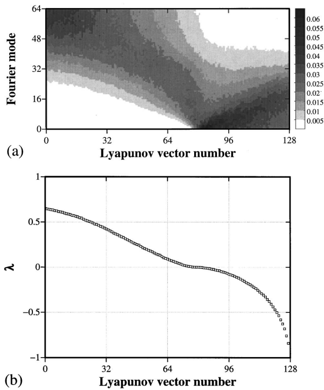
FIG. 11. Power spectrum (a) and Lyapunov spectrum (b) at u=0.3 , deep inside the chaotic phase T2. The dominant contribution to the Lyapunov vectors corresponding to small \lambda comes from the long wavelength Fourier modes, but due to the contribution from mid-wavelength modes the singularity in the exponent density becomes much weaker. Lattice size is 128.
