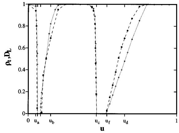
FIG. 9. Lyapunov dimension D_L (●) and turbulent set measure \rho_i (+) as functions of the conserved quantity u , calculated on the lattices with 128 and 2048 sites, respectively. Only the values in the chaotic state are shown if two attractors coexist.
