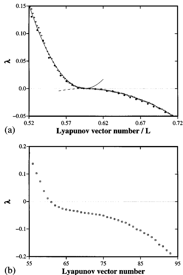
FIG. 14. ‘‘Slow’’ part of Lyapunov spectra of the unperturbed system and the system with nonlinear ‘‘dissipative’’ perturbation. (b) The spectrum of the perturbed system ( u_0=0.8 , L=128 ) with \epsilon=0.2 appears to be shifted downwards and tilted with respect to (a) the spectrum of the unperturbed system ( u=0.8 ). Here the data for two lattice sizes, L=128 ( \bullet ) and L=512 ( + ), is superimposed to show the finite-size effects. The density of exponents is seen to be singular on both the positive and negative side. The solid and the dashed lines give the quadratic fit provided by eqs. (67) and (65), respectively.
