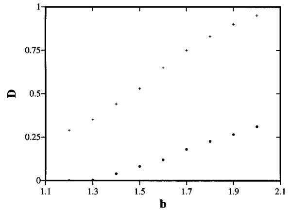
FIG. 13. Effective diffusion constant as a function of parameter b . a = 0.4 and u = 0.8 . The values of D_{Is} (+) are determined using the Lyapunov spectrum of the lattice with L = 128 , assuming \alpha = 0.5 . D_{sf} (●) is obtained from the dynamic structure function calculated for k = 0.01\pi on the lattice with L = 2048 .
