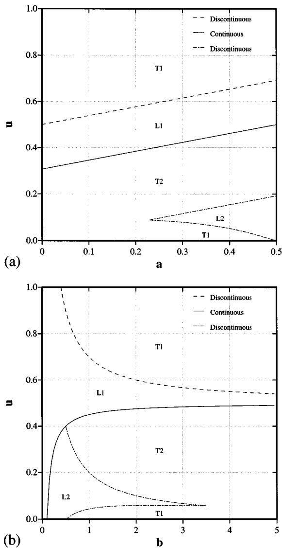
FIG. 1. Cross-sections of the phase diagram in a three-dimensional parameter space (a) u vs a at b=1.3 ; (b) u vs b at a=0.4 . The solid line corresponds to a continuous phase transition. The dashed and the dotted lines denote the phase boundaries where discontinuous phase transitions between chaotic and non-chaotic states occur.
