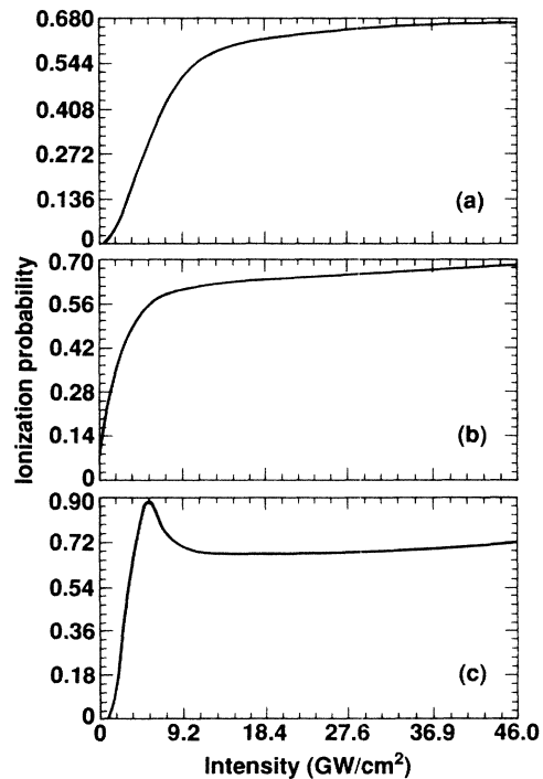
FIG. 1. Probability of ionization as a function of laser intensity and resonance detuning through the 3p intermediate state: (a) detuning = -0.2 \text{ cm}^{-1} , (b) detuning = 0.0 \text{ cm}^{-1} , and (c) detuning = 0.2 \text{ cm}^{-1} .
