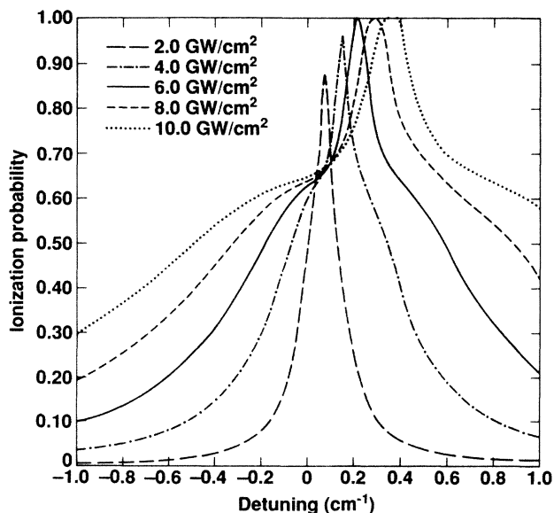
FIG. 2. Probability of ionization as a function of detuning for different laser intensities through the 3p intermediate state and a pulse duration of 10 ns.
