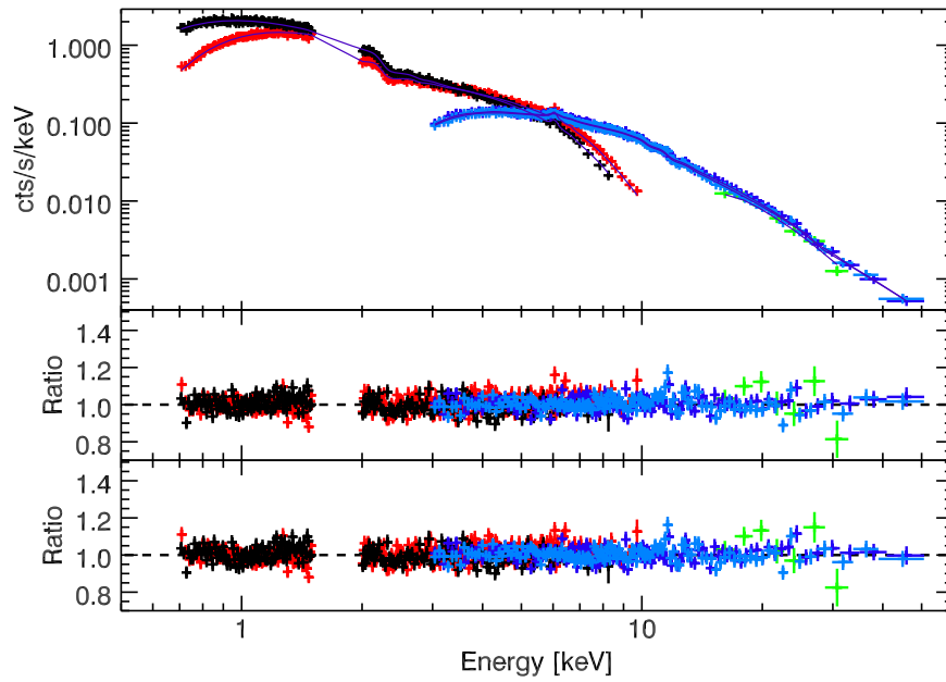
Figure 5. Data (top panel) and residuals to the best-fitting pexmon (middle panel) and eqpair (bottom panel) model. In all cases, the Suzaku -XIS data are shown in black and red, the Suzaku -PIN data in green, the NuSTAR data in blue, and the model in the top panel is shown in purple. The data have been rebinned in xspec for clarity.
