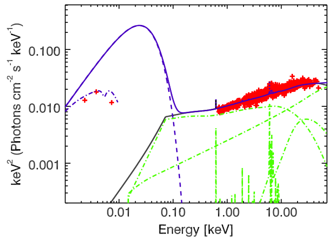
Figure 7. Spectral Energy Distribution of 3C 390.3 from Swift -UVOT, Suzaku -XIS, and NuSTAR . The data are shown in red. The models overlaid are (a) the X-ray Comptonization model shown in Table 2 (black solid line) and (b) the modified Comptonization model shown in Table 3 (blue solid line). The effects of Galactic absorption and reddening are not included in the plotted models, but the effect of intrinsic reddening is shown in the case of the modified Comptonization model as the dotted–dashed blue curve. The dashed blue curve shows the multi-color disk blackbody unaffected by reddening. The other individual model components are shown in green.
