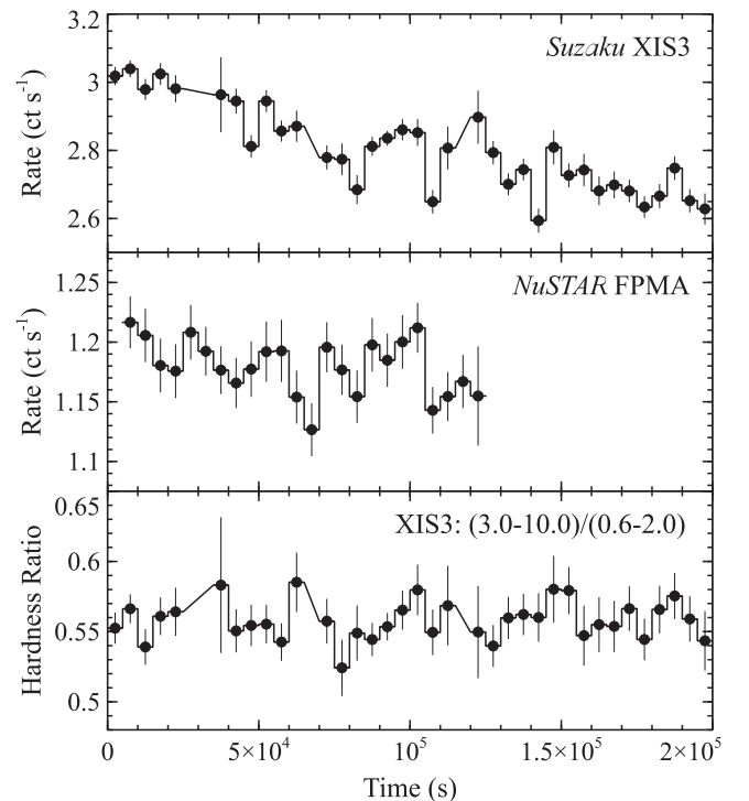
Figure 1. Suzaku -XIS (top panel) and NuSTAR (middle panel) light curves in 5 ks binning. A slight flux decrease throughout the observations is apparent. The hardness ratio within the Suzaku -XIS band (bottom panel) stays constant during this decline.
