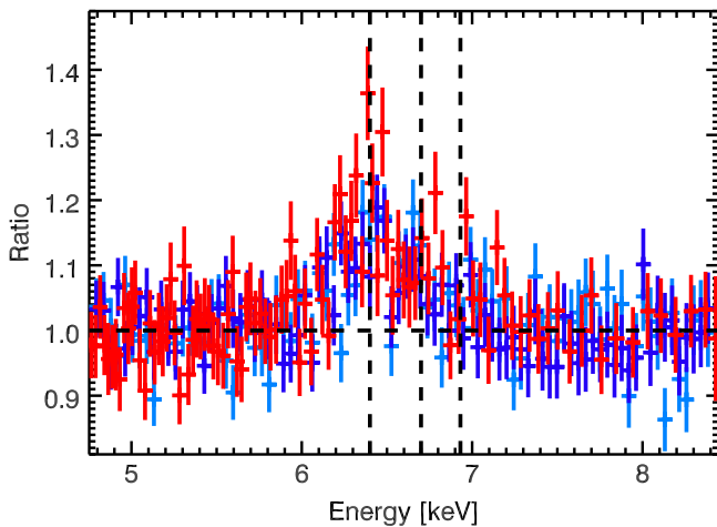
Figure 6. Suzaku -XIS (red) and NuSTAR FPMA (light blue) and FPMB (blue) ratio to a simple power law fitted to the 4.5–5.5 and 6.5–8.0 keV plotted in the rest frame of 3C 390.3. Also indicated by the three vertical lines are the rest frame positions of Fe K\alpha , Fe xxv, and Fe xxvi. NuSTAR is binned to a signal to noise of 10 while Suzaku is binned to a signal to noise of 17 to agree better with the resolution of NuSTAR .
