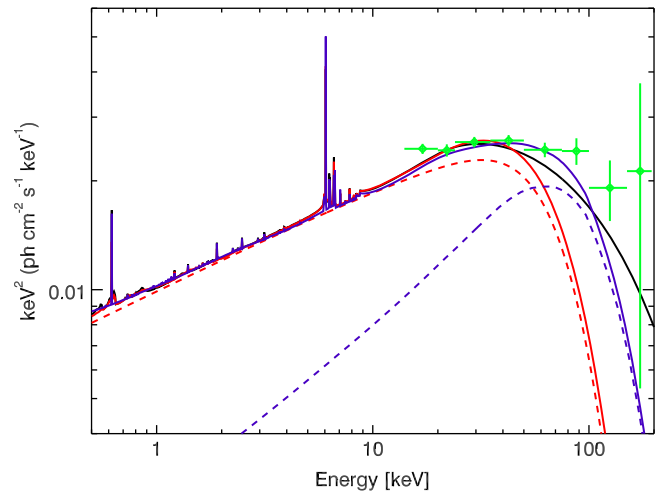
Figure 8. 70 month Swift -BAT spectrum with overlaid unabsorbed best-fit models for the three different continua considered here: pexmon (black curve), compTT (red curve), and eqpair (purple curve). The dashed curves show only the primary continuum for the two Comptonization fits.
