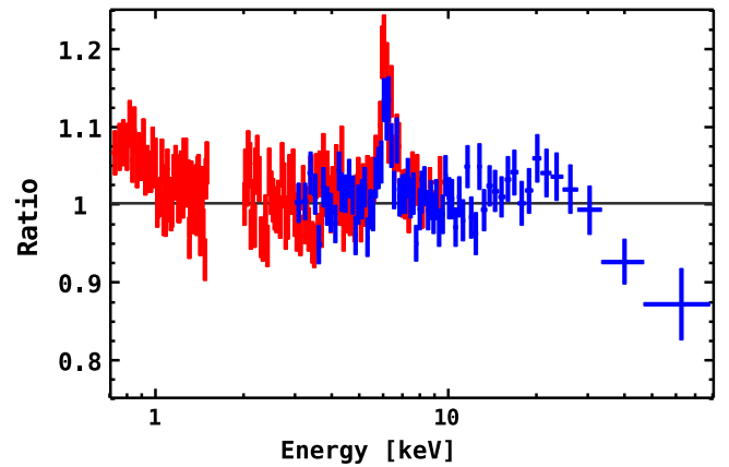
Figure 2. Residuals to a simple absorbed power law fitted to the 2–4 and 8–10 keV bands for the front-illuminated Suzaku -XIS (red) and NuSTAR -FPMA (blue). The data have been rebinned strongly for plotting.
