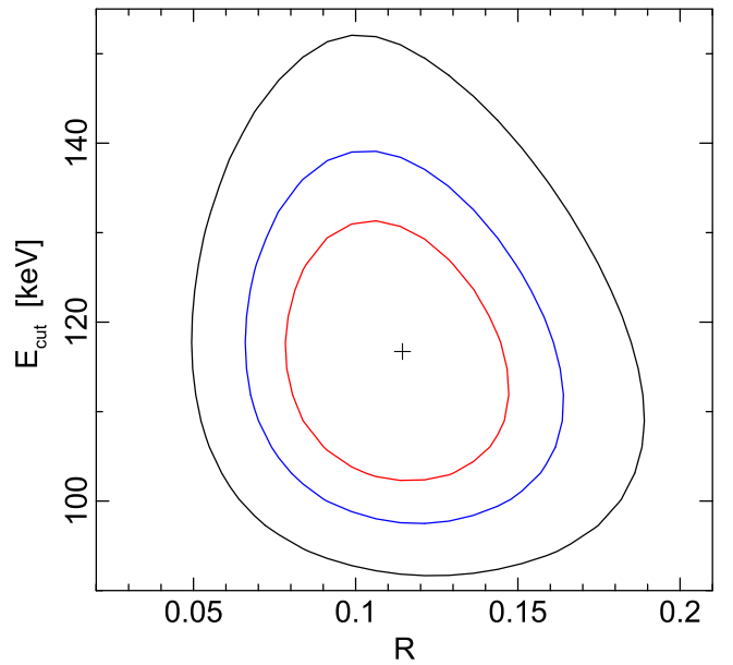
Figure 3. Confidence contour of the reflection fraction R and the high energy cut-off energy E_{\text{cut}} .
