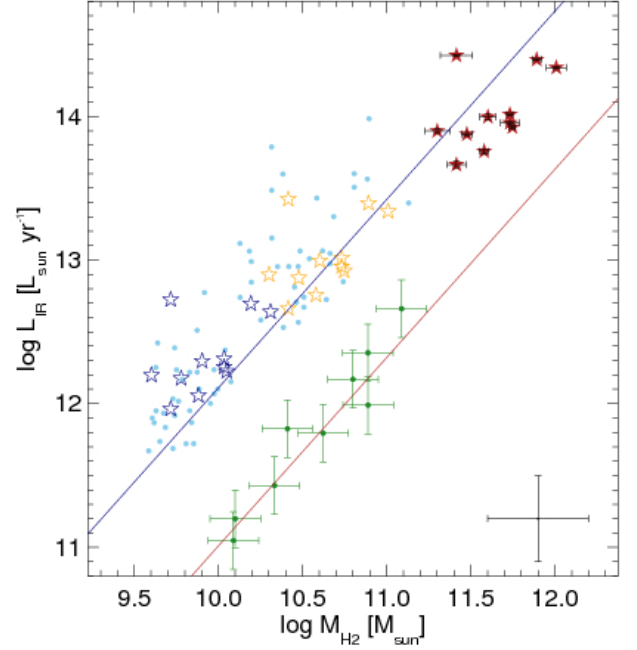
Fig. 10. Left: Infrared luminosities ( L_{\text{IR}} ) as a function of molecular gas mass for our sources. Red, yellow, and purple stars indicate the measured values (uncorrected for gravitational amplification), and the same values corrected by fiducial lensing factors of 10 and 50, respectively. In agreement with the dust-to-gas ratios discussed in Sect. 9 we adopt the classical “ULIRG” conversion factor \alpha_{\text{CO}} = 0.8 M_{\odot}/(\text{K km s}^{-1} \text{pc}^2) for all sources. The blue and red line indicate the relationships for starbursts and “main-sequence” galaxies emphasized by Daddi et al. (2010). Small dots show the low- and high- z samples of Daddi et al. (2010) for comparison. Light blue dots along the upper line show low- and high- z ULIRGs and SMGs, respectively. The filled dark green dots (with error bars) are BzK galaxies at z \sim 2 ; for details of these samples see Daddi et al. (2010). All error bars include the measurement uncertainties. The black cross in the lower right corner of the plot shows a fiducial factor 2 in statistical uncertainties.
