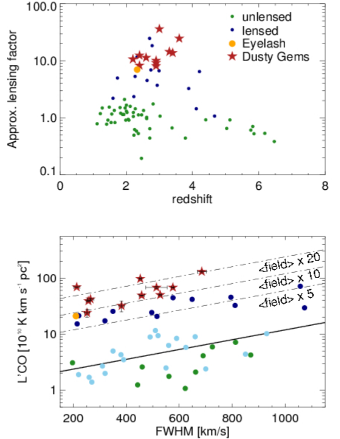
Fig. 6. Top: Order-of-magnitude estimate of the gravitational magnification factor derived from the dust temperature and FIR luminosity of our sources compared to FIR/submm galaxies in the field (see Sect. 6.2 for details). Bottom: CO emission-line luminosity as a function of FWHM line width, using the same symbols as in the top panel, with additional light blue dots showing those sources of Bothwell et al. (2013), which are neither gravitationally lensed nor AGN hosts. The solid and dashed lines show the best linear fit to the sample of field galaxies, as well as shifts of this line corresponding to magnification factors of 5, 10, and 20. Error bars show the 1\sigma uncertainties of our single-component Gaussian line fits.
