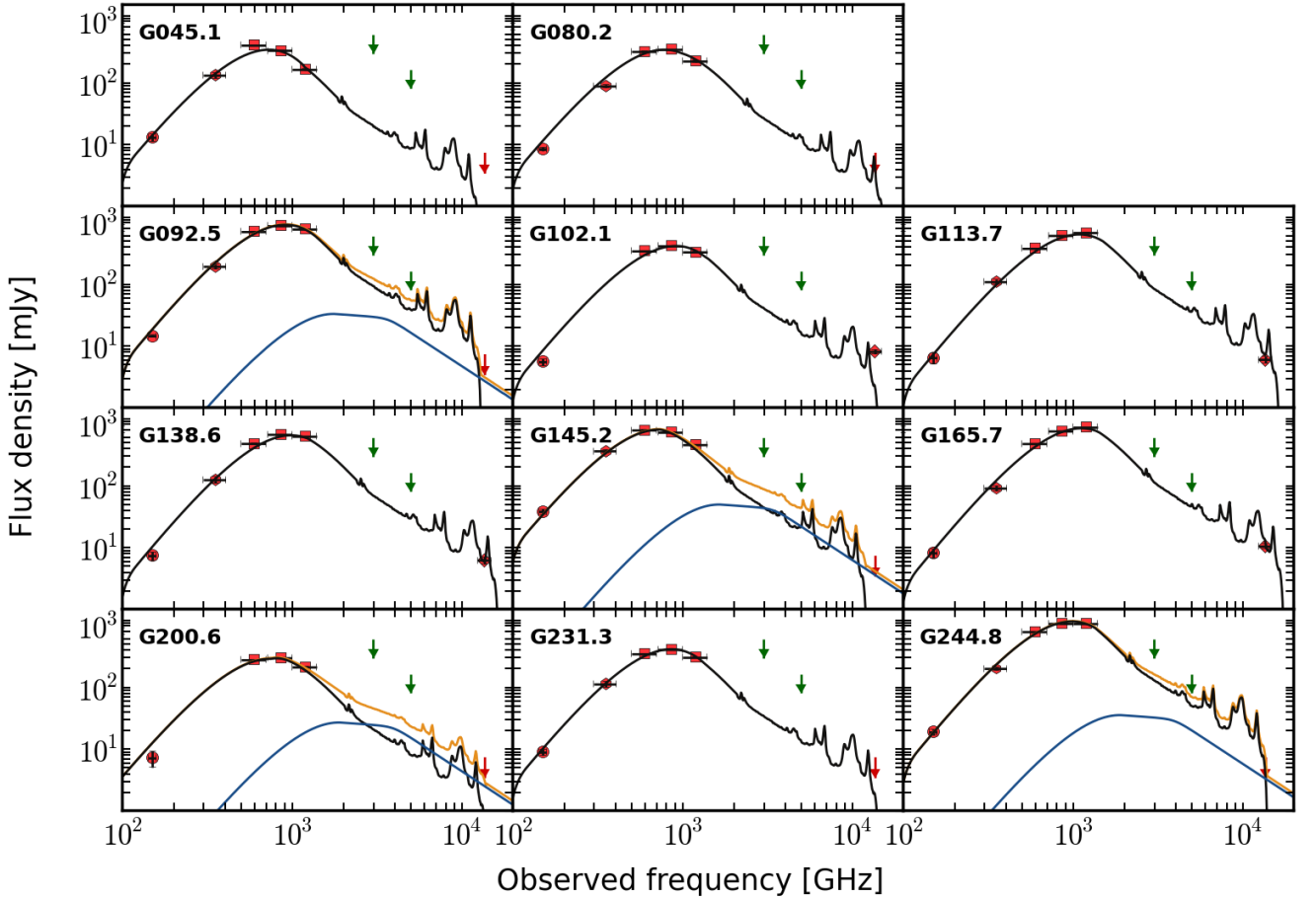
Fig. 7. Infrared-to-millimetre spectral energy distributions of all of our 11 sources obtained using DecompIR (Mullaney et al. 2011). Red dots show our data points, where the error bars along the abscissa indicate the width of each band. The error bars along the ordinate are often smaller than the symbol size. Green downward arrows show the 90% completeness limit of the IRAS all-sky survey at 60 and 100 \mu\text{m} , respectively. Red downward arrows at 22 \mu\text{m} show the 5\sigma upper limits provided by the WISE catalogs, where the counterparts were fainter than the 5.4 mJy flux limit of the WISE catalog. Black, blue, and yellow lines show the starburst and AGN component (if an AGN was fitted), and the sum of both, respectively.
