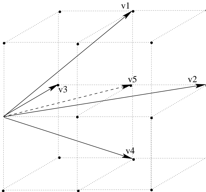
Figure 1: The fan for the resolution of the \mathbb{Z}_2 orbifold of \mathcal{O}_{-1} + \mathcal{O}_{-1} \rightarrow \mathbb{P}^1 .
