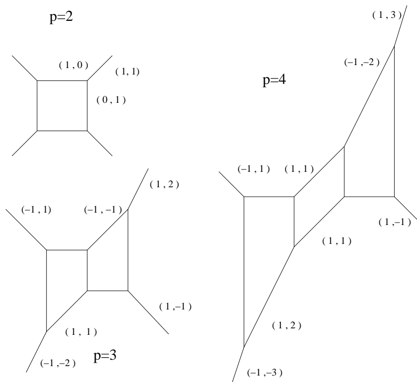
Figure 2: The toric web diagrams of the large- N dual of T^*(S^3/\mathbb{Z}_p) for some values of p .
