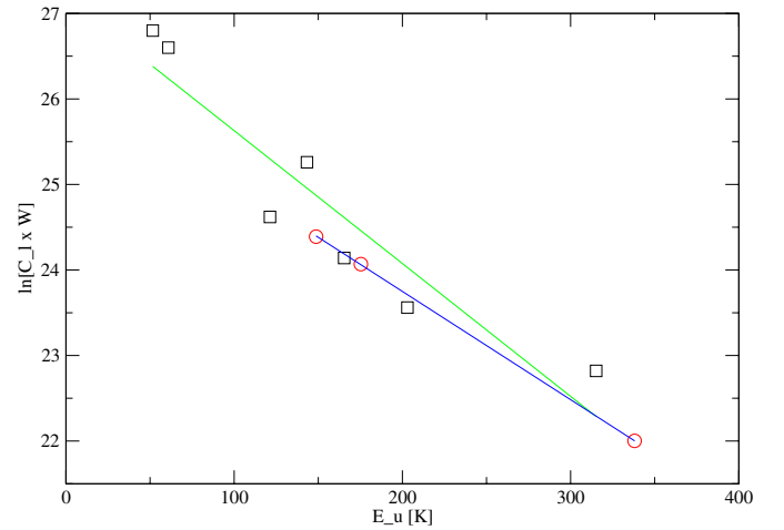
Fig. 11. Population diagram for CH 3 OH-A (squares) and CH 3 OH-E (circles). E_u is the energy of the upper level, C_l a constant of the line and W is the integrated main beam line intensity.
