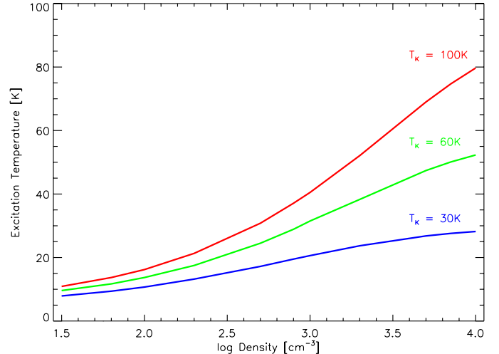
Fig. A.1. Excitation temperature vs. cloud density for the 487 GHz O 2 transition resulting from RADEX multi-transition analysis, using three values of kinetic temperature: 30, 60 and 100 K.
