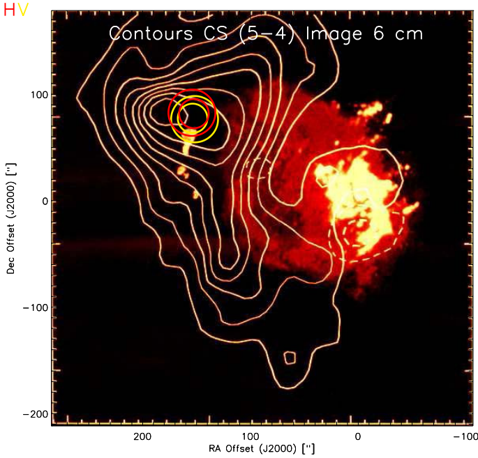
Fig. 1. Sgr A +50 \text{ km s}^{-1} Cloud, delineated by the integrated emission ( +20 to +80 \text{ km s}^{-1} ) in the CS(5–4) line (contours), superimposed upon a 6 cm continuum map of the Sgr A Complex (colour image – red: non-thermal Sgr A East, yellow: thermal Sgr A West and the four compact H II regions of which A is the northernmost, close to our observational position) (Serabyn et al. 1992). The FWHM Herschel 487 and 774 GHz beams, H (northernmost) and V polarizations, for the HOP observations we have carried out are indicated by red and yellow circles, respectively.
