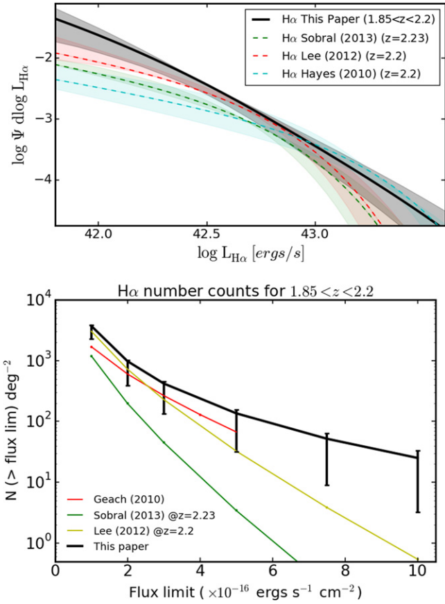
Figure 9. Top: The collapsed H \alpha LLF at z \sim 2 derived using the best-fit [O III] LLF and the best-fit bivariate LLF parameters from Table 1. The shaded regions represent the 1\sigma deviations in the best-fit parameters. Bottom: The H \alpha number counts estimated for z \sim 2 from our H \alpha LF, along with estimates from other groups in the literature. The errors on our estimate accounts for the uncertainties in the best-fit parameters in addition to the normal Poisson errors. All number counts are corrected for survey incompleteness.
