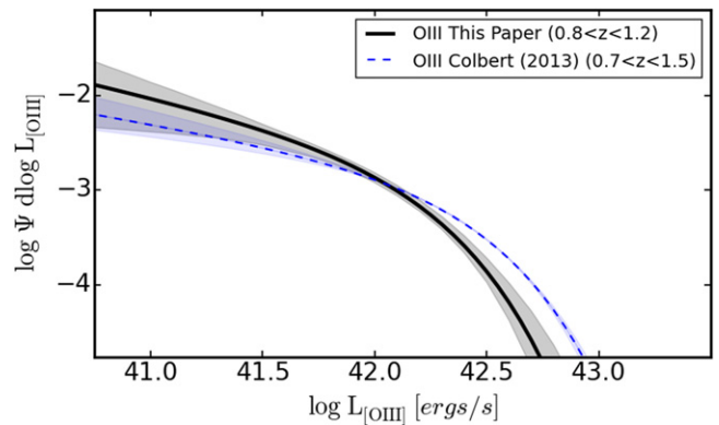
Figure 4. Collapsed [O III] LLF derived from the best-fit bivariate LLF from Figure 2 compared with the [O III] luminosity function from Colbert et al. (2013). The shaded regions represent the 1\sigma deviations in the best-fit parameters.
