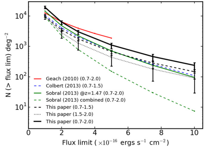
Figure 10. H \alpha number counts estimated for 0.7 < z < 2.0 , the relevant redshift range for future surveys to cover H \alpha . The redshift range for each estimate is reported in parenthesis in the legend. Our estimate (solid black) is split into two ranges: 0.7 < z < 1.5 (dashed black) and 1.5 < z < 2 (dotted black), which use the z \sim 1 and z \sim 2 H \alpha LFs, respectively. We also plot two estimates from Sobral et al. (2013): the solid green line represents the H \alpha number counts estimated using the H \alpha LF derived at z = 1.47 and the dashed green line represents the sum of number counts estimated over the redshift ranges 0.7–1.2, 1.2–1.85, and 1.85–2.0 using H \alpha LFs derived at z = 0.84 , 1.47, and 2.23, respectively. The errors on our estimate account for the uncertainties in the best-fit parameters in addition to the normal Poisson errors. All number counts are corrected for survey incompleteness.
