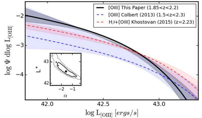
Figure 8. Best-fit [O III] LLF at z \sim 2 derived from WISP data plotted along with other estimates from the literature. The shaded regions represent the 1\sigma deviations in the best-fit parameters. The inset shows the joint-posterior distribution of \alpha and L^* from the MCMC analysis for our best-fit [O III] LF.
