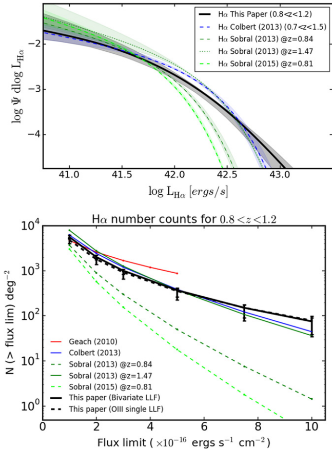
Figure 7. Top: the collapsed H \alpha LLF for 0.8 < z < 1.2 derived using the best-fit [O III] LLF in Figure 6 and the best-fit bivariate LLF parameters \beta , r , and \sigma_{\ln \text{H}\alpha} from Table 1. Bottom: the H \alpha number counts estimated for z \sim 1 from our H \alpha LF, along with estimates from other groups in the literature. The errors in our estimate account for the uncertainties in the best-fit parameters in addition to the normal Poisson errors. All number counts are corrected for survey incompleteness.
