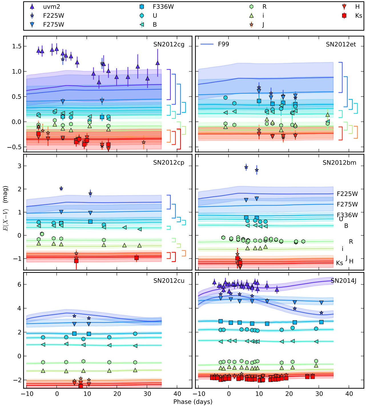
Figure 6. The observed colour excess, E(X - V) , against phase for all SNe and filters. The predicted colour excess from the SN2011fe template and the fitted F99 law, presented in Table 5, is shown with solid lines and the regions surrounding them mark the adopted intrinsic colour uncertainties. The uncertainties are also indicated by open brackets for the three SNe with the least reddening. The phase, p = (t - t_B^{\max})/s_B , was calculated based on the fitted t_B^{\max} and s_B values from Table 5. The apparent E(X - V) time-dependence of the F225W filter for e.g. SN2014J originates from the red tails of these filters which causes the observed colour excess to vary with the intrinsic colour of the source.
