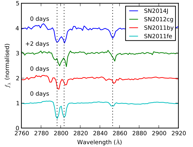
Figure 17. Mg II at \lambda\lambda 2796, 2803 Å and Mg I at \lambda\lambda 2853 Å marked by dotted lines in STIS spectra of four SNe with different reddening. The continua of the unsmoothed spectra are normalised and offset for clarity. Above the respective spectra, the phases are indicated at which the spectra were taken.
