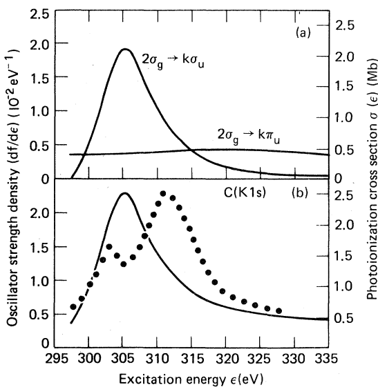
FIG. 9. (a) As in Fig. 2(a) for 2\sigma_g \rightarrow k\sigma_u and k\pi_u photoionization; (b) as in Fig. 2(b) for C1s K -edge photoionization in \text{CO}_2 ; \bullet , electron-impact data (Ref. 19) normalized to the calculated values at \sim 300 eV.
