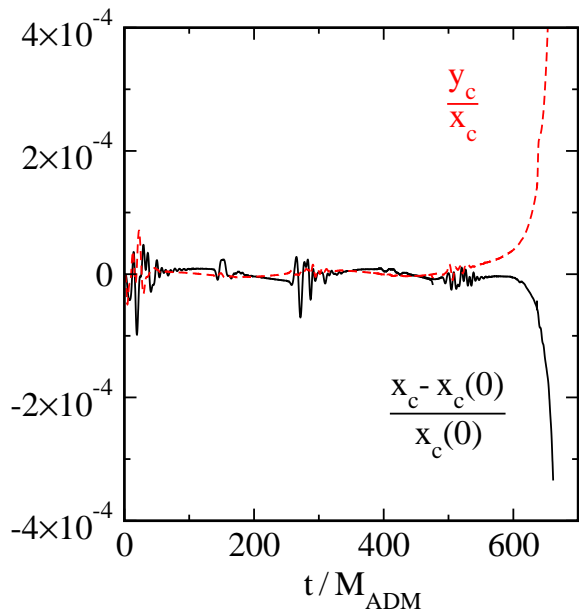
FIG. 10: Evolution of the apparent horizon center of one black hole for a binary black-hole evolution using a feedback system that adjusts the moving coordinate frame to control both the parameters y_c/x_c and [x_c - x_c(0)]/x_c(0) . Compare to Figs. 6 and 8.
