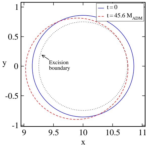
FIG. 7: Moving coordinate frame representation of an equatorial slice through the apparent horizon of one of the black holes for the evolution of Fig. 6. The evolution is terminated when the apparent horizon approaches the excision boundary (dotted curve) near the right side of this figure.
