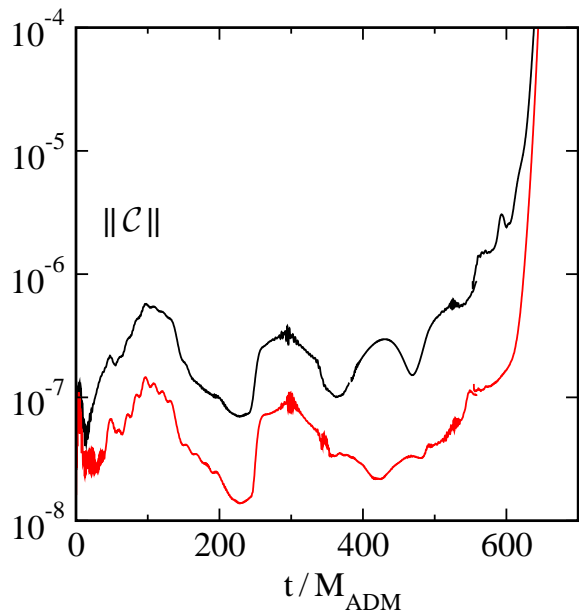
FIG. 12: Constraint violations \|\mathcal{C}\| for the binary black-hole evolution of Fig. 10. The two curves represent two numerical resolutions, the upper curve has about 64^3 collocation points, while the lower curve has about 76^3 collocation points.
