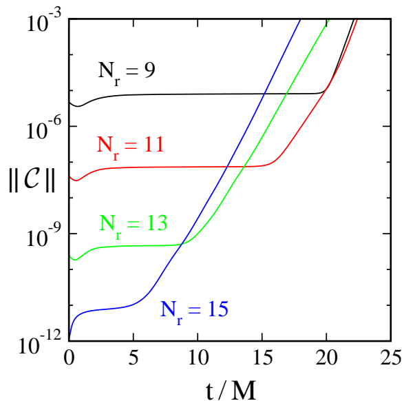
FIG. 2: Constraint violations in dual-coordinate-frame evolutions of Schwarzschild, with comoving coordinates that rotate uniformly with angular velocity \Omega = 0.2/M . Angular filtering (see text) is performed on the inertial frame components.
