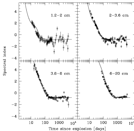
FIGURE 3. The spectral index ( \alpha ; S \propto \nu^{+\alpha} ) evolution for SN 1993J between 1.2 and 2 cm (top left), between 2 and 3.6 cm (top right), between 3.6 and 6 cm (bottom left), and between 6 and 20 cm (bottom right). As in Figure 2 the lines represent the best fit combined synchrotron self-absorption (SSA) and thermal, free-free absorption (FFA) model as described in the text and by Weiler et al. [42].
