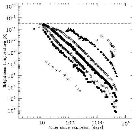
FIGURE 4. The brightness temperature ( T_B ) evolution for SN 1993J for, from left to right, 0.3 ( \times ), 1.2 (filled square), 2 (open square), 3.6 (filled circle), 6 (open triangle), 20 (filled triangle), 49 (*), and 90 (open diamond) cm corrected for extended, free-free absorption flux density suppression at early times as described in the text and by Weiler et al. [42]. The horizontal dashed line denotes the limiting value of T_B \simeq 3 \times 10^{11} K [27], which is not exceeded at any frequency.
