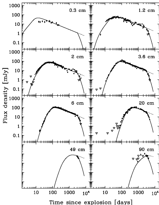
FIGURE 2. The radio light curves for SN 1993J are plotted from left to right and top to bottom at 0.3, 1.2, 2, 3.6, 6, 20, 49, and 90 cm. The lines represent the best fit combined synchrotron self-absorption (SSA) and thermal, free-free absorption (FFA) model as described in the text and by Weiler et al. [42] with an exponential flux density decline after day 3100 with an e-folding time of 1100 days. Upper limits ( 3\sigma ) are shown as open inverted triangles).
