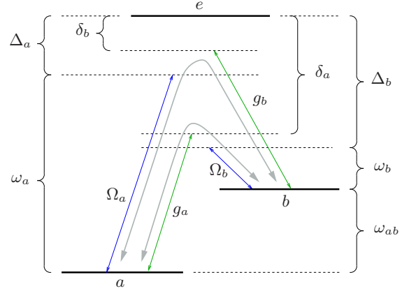
FIG. 1: Level structure, driving lasers and relevant couplings to the cavity mode to generate effective \sigma^x\sigma^x - and \sigma^y\sigma^y -couplings for one atom. The cavity mode couples with strengths g_a and g_b to transitions |a\rangle \leftrightarrow |e\rangle and |b\rangle \leftrightarrow |e\rangle respectively. One laser with frequency \omega_a couples to transition |a\rangle \leftrightarrow |e\rangle with Rabi frequency \Omega_a and another laser with frequency \omega_b to |a\rangle \leftrightarrow |e\rangle with \Omega_b . The dominant 2-photon processes are indicated in faint gray arrows.
