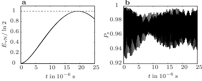
FIG. 4: a The von Neumann entropy E_{vN} of the reduced density matrix of 1 effective spin in multiples of \ln 2 and b the purity of the reduced state of the effective spin model for 2 cavities where J_z = 0.042\text{MHz} .
