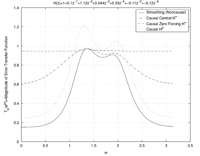
Fig. 3. Inversion of the noisy channel H(z) = 1 + .1z^{-1} + 1.12z^{-2} + .044z^{-3} + .33z^{-4} - .11z^{-5} - .12z^{-6} .
