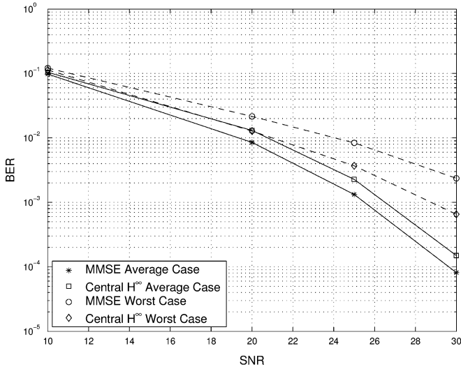
Fig. 4. Average and worst case BER performances of MMSE and the central H^\infty equalizers.
