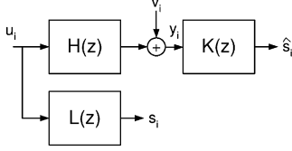
Fig. 2. A general estimation problem.
