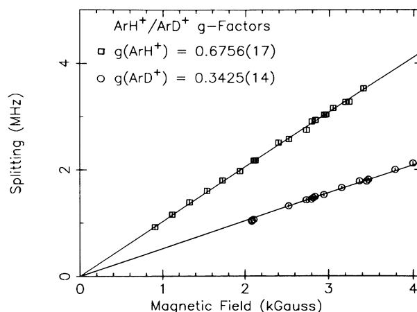
FIG. 2. Rotational Zeeman-effect splitting vs magnetic field for \text{ArH}^+ and \text{ArD}^+ .
