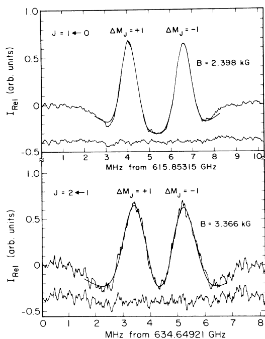
FIG. 1. Rotational spectra of \text{ArH}^+ (top) and \text{ArD}^+ (bottom) showing the magnetic splitting. The fitted lines are superimposed on the observed spectrum, and the residuals are shown below.
