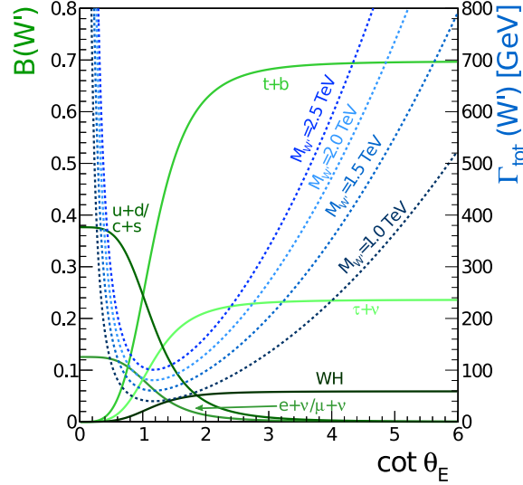
Figure 1: Branching fractions (left-hand scale and solid lines) and total width (right-hand scale and dotted lines) for W' decays in the NUGIM, as calculated in Refs. [2, 10, 11]. For \cot \theta_E = 1 the values are the same as those in the SSM, rescaled to accommodate the WH decay channel.
