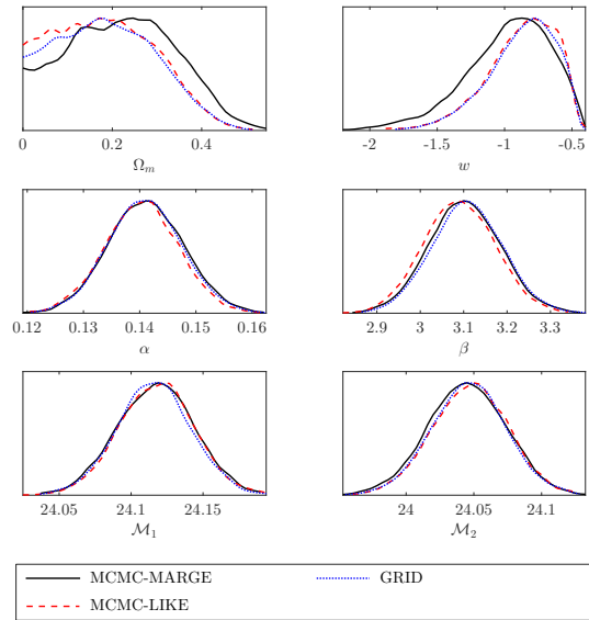
Figure 2. Mean likelihood pdf's of the parameters from the cosmological fit for the MCMC sets comparing with the GRID set, using all 740 SNe from the JLA data set. Black solid lines represent the MCMC-MARGE set; red dashed lines represent the MCMC-LIKE set; blue dotted lines represent the GRID set.
