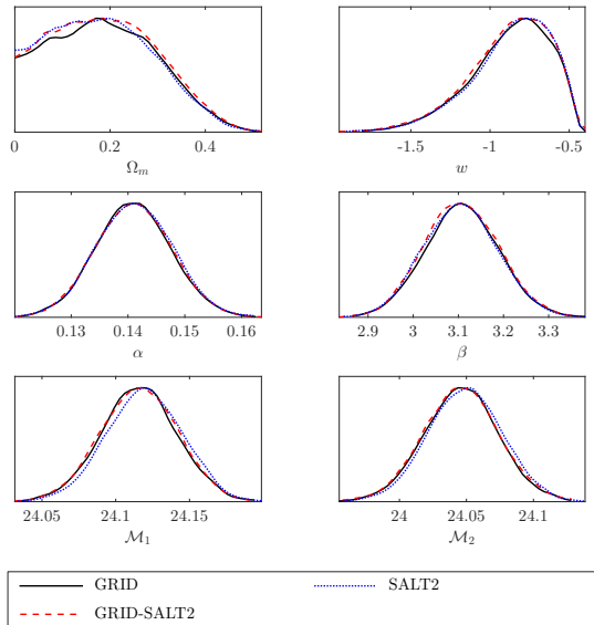
Figure 1. Mean likelihood pdf's of the parameters for the cosmological fit for the grid sets, using all 740 SNe from the JLA data set. Black solid lines represent the GRID set; red dashed lines represent the GRID-SALT2 set; blue dotted lines are for the SALT2 set.
