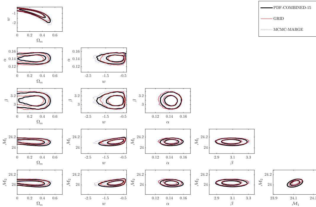
Figure 6. Joint confidence level contour plots from the cosmological fit with and without sampling of the SN Ia lightcurve parameter pdf's, using 729 SNe Ia from the JLA data set (excluding 11 problematic ones). The contours are 68% and 95% confidence levels. Thick black solid contours are results from sampling 15 points on each pdf (PDF-COMBINED-15); thin red solid contours are results from using the GRID set; blue dotted contours are results from using the MCMC-MARGE set, without pdf sampling.
