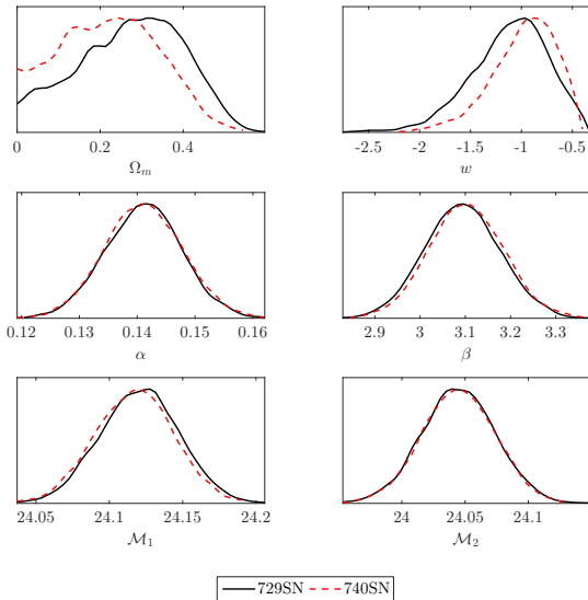
Figure 3. Mean likelihood pdf's of the parameters from the cosmological fit for different numbers of SNe Ia using the MCMC-MARGE set. Black solid lines show the results from 729 SNe excluding the 11 problematic SNe; red dashed lines represent the whole SNe sample including all 740 SNe from the JLA data set.
