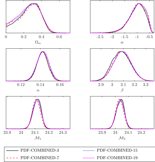
Figure 4. Mean likelihood pdf's of the parameters from the cosmological fit with sampling of the SN Ia lightcurve parameter pdf's, using 729 SNe Ia from the JLA data set (excluding 11 problematic ones). Black solid lines are results from sampling 3 points on each pdf (PDF-COMBINED-3); red dashed lines are results from sampling 7 points on each pdf (PDF-COMBINED-7); blue dotted lines are results from sampling 15 points on each pdf (PDF-COMBINED-15); magenta dash-dotted lines are results from sampling 19 points on each pdf (PDF-COMBINED-19).
