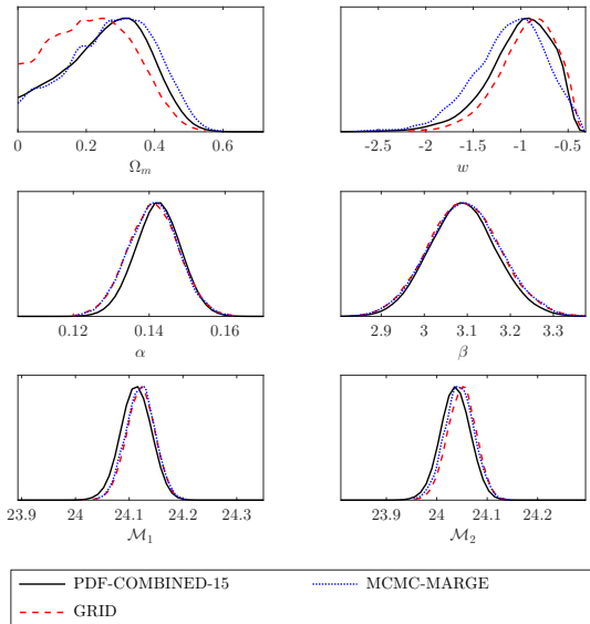
Figure 5. Mean likelihood pdf's of the parameters from the cosmological fit with and without sampling of the SN Ia lightcurve parameter pdf's, using 729 SNe Ia from the JLA data set (excluding 11 problematic ones). Black solid lines are results from sampling 15 points on each pdf (PDF-COMBINED-15); red dashed lines are results from using the GRID set; blue dotted lines are results from using the MCMC-MARGE set, without pdf sampling.
