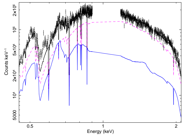
Figure 5. Decomposed RELXILL model spectrum for XMM-Newton RGS1 showing the reflection component (solid blue) and power law continuum (dashed purple). The RELXILL component is not shown to illustrate the model's ability to fit the O VIII line.
