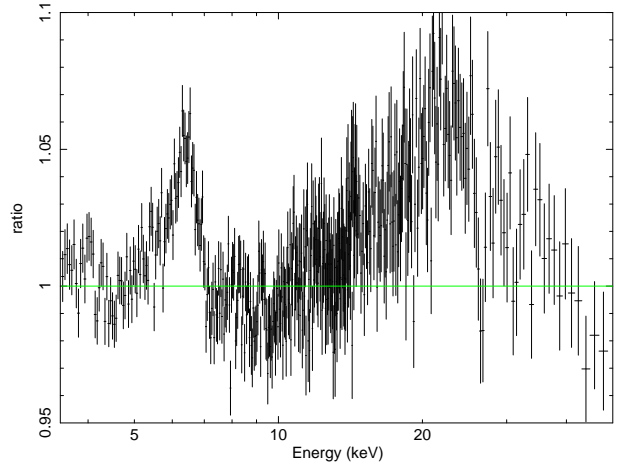
Figure 1. Ratio of the data to the continuum model for NuSTAR observation of 1RXS J180408. A simple cut-off power law was fit over the energies of 3.5-5 keV, 8-15 keV, and 30.0-50.0 keV. The iron line region from 5-8 keV and reflection hump was ignored to prevent the feature from skewing the fit. We ignore the region above 15 keV in this fit due to the presence of a X-ray reflection hump that peaks between 20-30 keV. The data was rebinned for plotting purposes.
