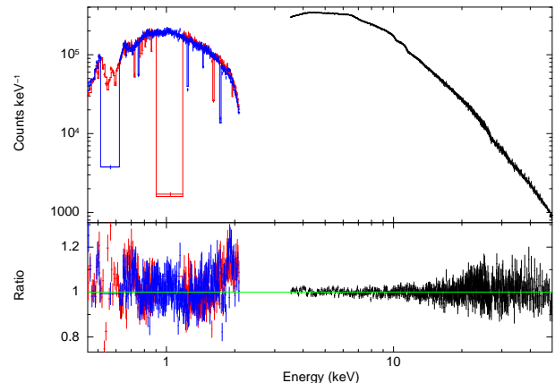
Figure 6. Joint fit of RGS and NuSTAR with \text{TBNEW}^*(\text{RELXILL}+\text{GAUSS}+\text{GAUSS}+\text{RELLINE}) ( \chi^2_{\text{red}} = 1.34 ). The additional RELLINE parameter is needed to model the He-like O VII line. Gaussians were fit at 10.1 keV and 11.5 keV to account for instrumental response features. Spectrum has been rebinned for plotting purposes. Parameter values can be seen in the fifth column of Table 1.
