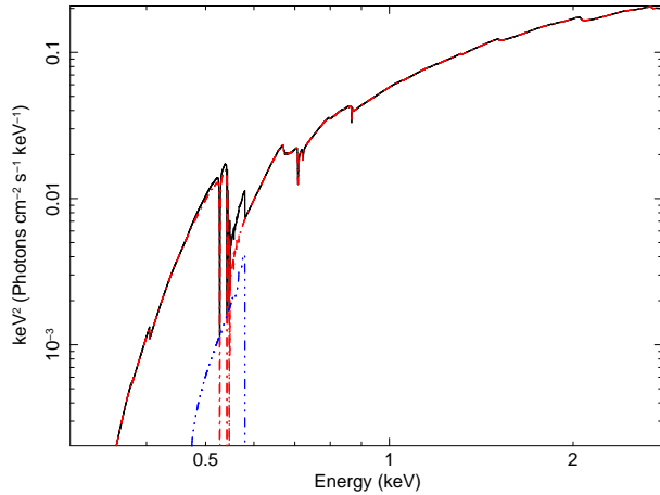
Figure 4. Unfolded model spectrum for XMM-Newton RGS. The blue component corresponds to RELXILL. The red component illustrates RELXILL which includes the power law.
