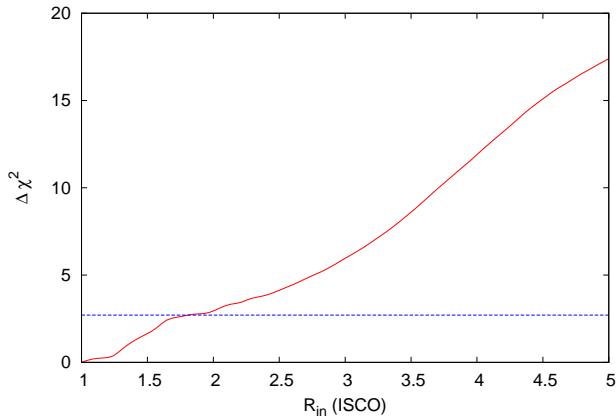
Figure 7. The change in goodness-of-fit versus inner disk radius for the NuSTAR +RGS column in Table 1 taken over 50 evenly spaced steps generated with XSPEC “steppar”. The inner disk radius was held constant at each step while the other parameters were free to adjust. The blue dashed line shows the 90% confidence level.
