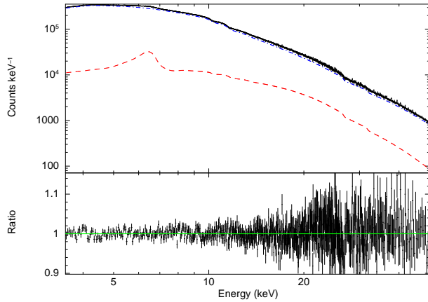
Figure 2. NuSTAR spectrum fit with \text{TBNEW}*(\text{RELXILL}+\text{GAUSS}+\text{GAUSS}) ( \chi^2_{\text{red}} = 1.05 ). Gaussians were fit at 10.1 keV and 11.5 keV to account for instrumental response features. The red dashed line shows the reflection spectrum from the RELXILL model. The blue dot-dash line shows the power law component within the RELXILL model. The lower panel shows the ratio of the data to model. Spectrum has been rebinned for plotting purposes. Parameter values can be seen in the third column of Table 1.
