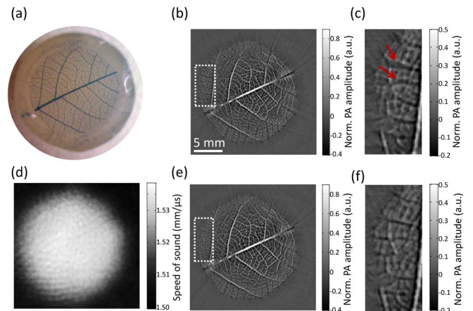
Fig. 5. Experimental results of a leaf phantom. (a) Photograph of the skeleton leaf embedded in an agar gel with SOS of 1.535 mm/μs. (b) PACT image reconstructed using a constant average SOS, which was optimized for image sharpness. (c) Zoomed-in view of the veins within the dashed box indicated in (b). (d) SOS map obtained from USCT measurement. (e) PACT image reconstructed using the SOS map in (d). (f) Zoomed-in view of the veins within the box indicated in (e).
