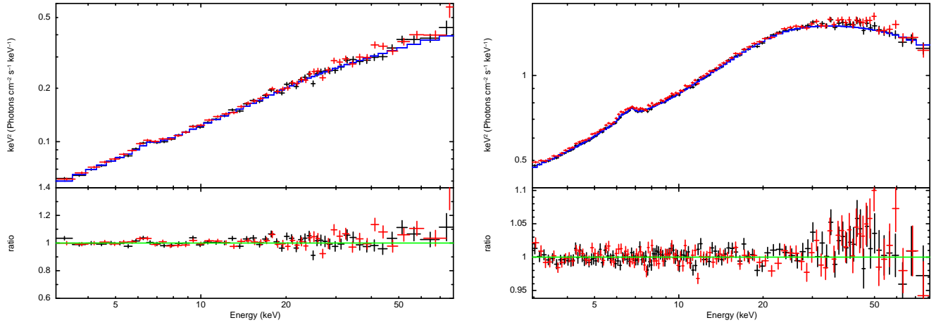
FIG. 3.— NuSTAR spectra of GS 1354–645, fit with the “relxill” relativistically blurred disk reflection model. The FPMA is shown in black, the FPMB is shown in red, and the model for the FPMA is shown in blue. The data in each panel have been rebinned for visual clarity. LEFT : The spectrum of Obs. 1 is shown. The data are consistent with reflection from a radially truncated accretion disk. RIGHT : The spectrum of the brighter Obs. 2 is shown. The best fit requires a very high black hole spin parameter.
