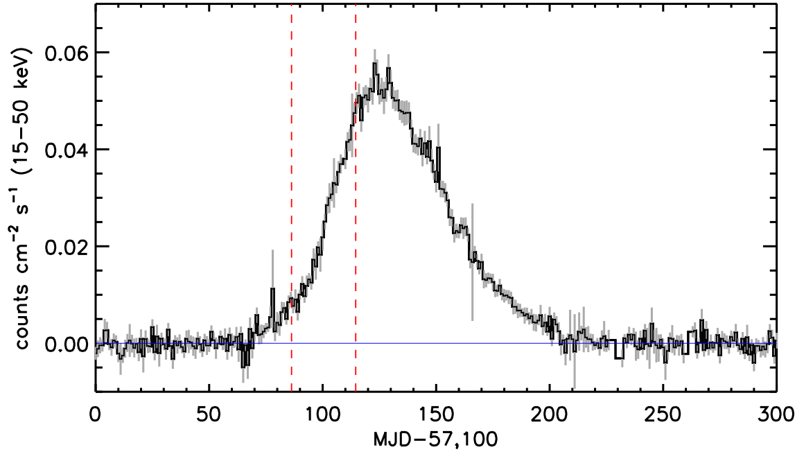
FIG. 1.— The Swift /BAT light curve of the 2015 outburst of the black hole GS 1354–645. The data points represent the average flux over a span of one day. The red, dashed, vertical lines indicate the start time of the two NuSTAR observations considered in this work, referred to as Obs. 1 and Obs. 2. The outburst is qualitatively consistent with a fast rise, exponential decay (FRED) profile.
