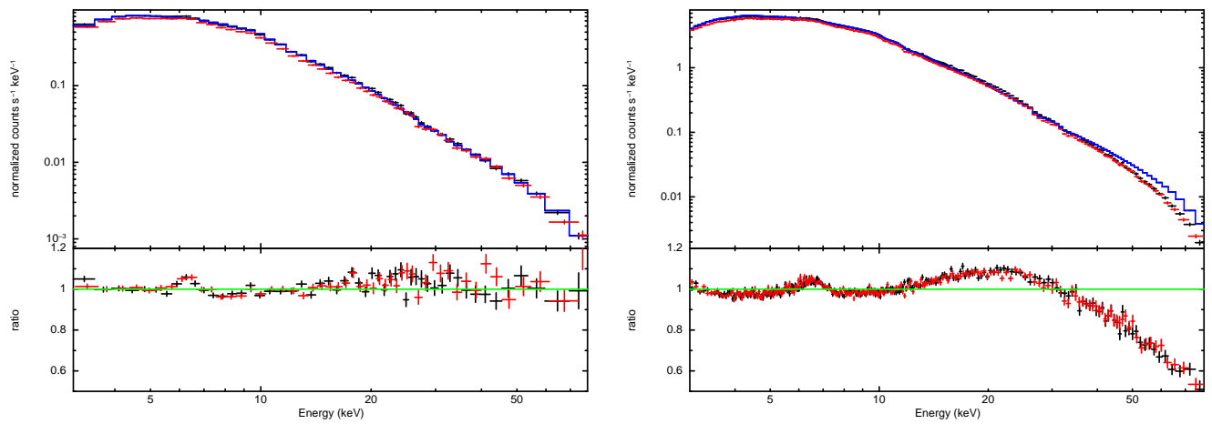
FIG. 2.— NuSTAR spectra of GS 1354–645, fit with a fiducial power-law continuum. The FPMA is shown in black, the FPMB is shown in red, and the model for the FPMA is shown in blue. The data in each panel have been rebinned for visual clarity. LEFT : The spectrum of Obs. 1 is shown. RIGHT : The spectrum of Obs. 2 is shown. This ratio reveals evidence of strong, broadened reflection consistent with illumination of the inner accretion disk.
