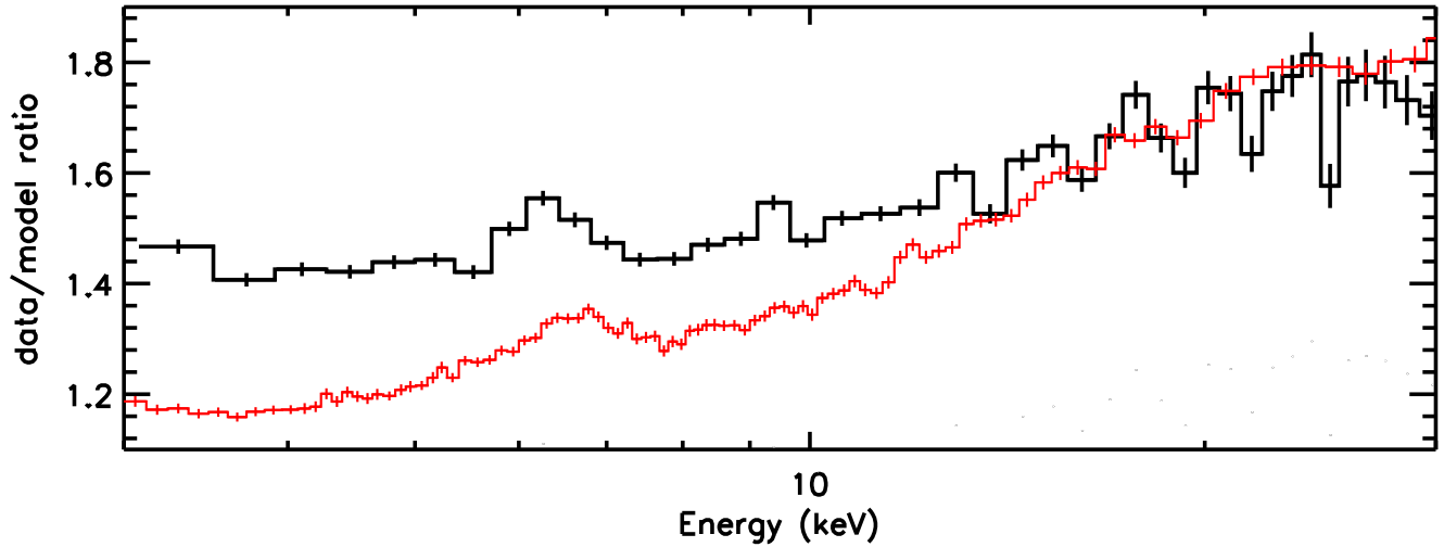
FIG. 4.— NuSTAR spectra from Obs. 1 (black) and Obs. 2 (red), after removing blurred disk reflection from the models detailed in Table 1. The unmodeled Fe K line in Obs. 2 extends down to 4–5 keV, consistent with a disk close to the ISCO around a spinning black hole. In contrast, the unmodeled Fe K line in Obs. 1 is relatively narrow. Only the FPMA spectra are shown, the ratio from Obs. 1 is multiplied by a factor of 1.4, and the data were binned for visual clarity.
