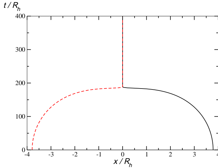
Fig. 1. BH trajectories for an equal-mass head-on collision of two non-spinning holes initially at rest in D = 7 dimensions. The collision takes place along the x axis.
