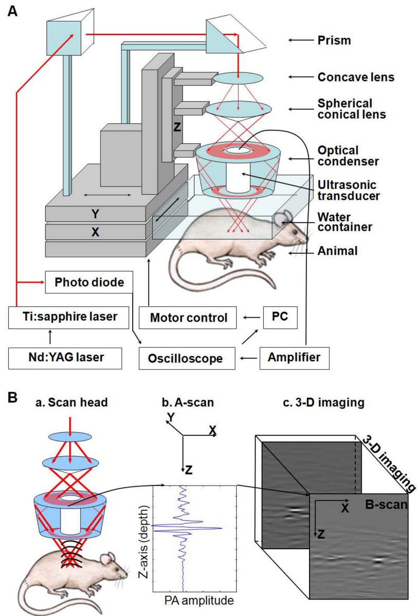
Figure 1. (A) Schematic of a deeply penetrating reflection-mode photoacoustic imaging system. (B) Image formation. A-scan: 1-D image and B-Scan: 2-D image. A B-scan is composed of multiple A-scans. Multiple B-scans form a 3-D image. PA: Photoacoustic.
