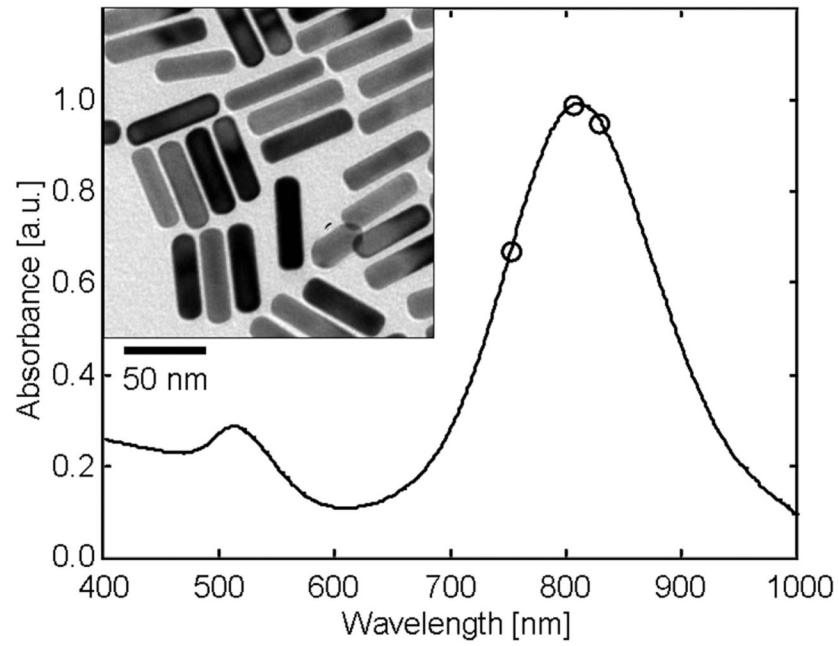
Figure 2. Absorbance of gold nanorods. Diameter: 10 nm, length: 41 nm, and a SPR peak wavelength: 807 nm. Normalized values are presented. Circles represent the wavelengths used for spectroscopic photoacoustic SLN mapping. Inset is a TEM image of the gold nanorods
