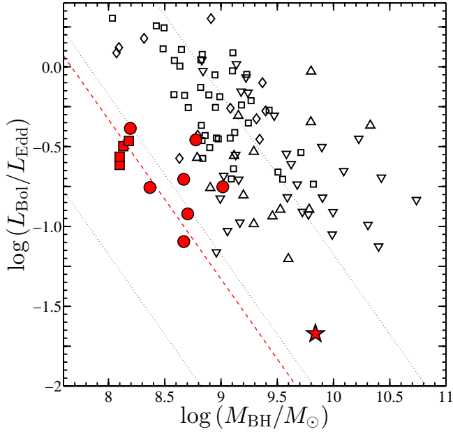
FIG. 5.— Accretion rate, in terms of L/L_{\text{Edd}} , vs. black hole mass, M_{\text{BH}} , for the sources studied here and several other relevant samples of high-redshift AGNs. The symbols are identical to those in Figure 4). The dotted lines represent constant bolometric luminosities of L_{\text{bol}} = 10^{45} , 10^{46} , and 10^{47} erg s ^{-1} . The red dashed line represents the flux limit of our study, L_{\text{bol}} = 7.8 \times 10^{45} erg s ^{-1} (at z = 3.5 ; see Section 2.1), which is most relevant for the z \simeq 3.3 sources. Some of the z \simeq 3.3 AGN fall below the flux limit, due to the host-light corrections. Compared to the combined sample of Shemmer et al. (2004) and Netzer et al. (2007), our sources exhibit lower masses but comparable accretion rates. With the exception of the extreme source CID-947 (red star), our sample lacks AGNs with high M_{\text{BH}} and low L/L_{\text{Edd}} (i.e., M_{\text{BH}} > 2 \times 10^9 M_{\odot} and L/L_{\text{Edd}} < 0.1 ).
