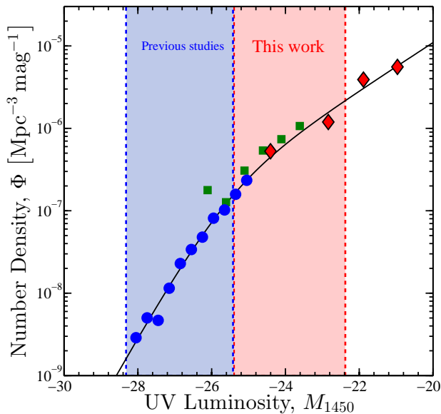
FIG. 1.— The luminosity function of unobscured AGNs at z \sim 3 - 3.5 , reproduced from the study of Masters et al. (2012), including the best-fit double power-law model (black line). The red diamonds represent COSMOS AGNs, similar to the parent sample from which our targets are drawn. Blue circles at higher luminosities are taken from the SDSS (Richards et al. 2006), while the green squares in the overlap region are taken from the SWIRE survey (Siana et al. 2008). Other samples and error bars from all data points are omitted for clarity. The shaded regions represent the luminosity regimes covered by our sample (red) and previous studies of M_{BH} and L/L_{Edd} in luminous z \sim 3 - 4 AGNs (blue; Shemmer et al. 2004; Netzer et al. 2007). Our sample probes a much more representative population of z \simeq 3.3 AGNs, with an integrated number density that is higher by a factor of about 25 than the previously studied objects.
