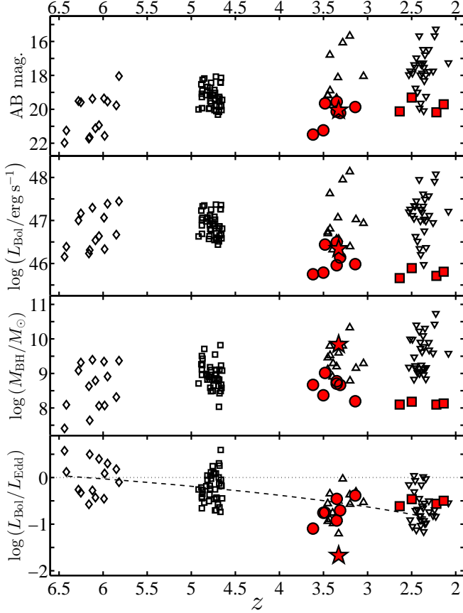
FIG. 4.— From top to bottom, trends of observed (NIR) brightness, L_{\text{bol}} , M_{\text{BH}} , and L/L_{\text{Edd}} for the available samples of unobscured AGNs at z > 2 , with reliable determinations of M_{\text{BH}} . The red symbols represent the measurements reported in this work, at z \simeq 3.3 and 2.4 (circles and squares, respectively). CID-947, which was analyzed in detail in Trakhtenbrot et al. (2015) , is highlighted by a star. The different black symbols represent other, optically selected sources, studied in the combined sample of Shemmer et al. (2004) and Netzer et al. (2007) , triangles at z \simeq 2.4 and \simeq 3.3 ; Trakhtenbrot et al. (2011) , squares at z \simeq 4.8 ; and the combined samples of Kurk et al. (2007) and Willott et al. (2010) , diamonds at z \simeq 6.2 . The dotted line in the bottom panel marks the Eddington limit, i.e., L/L_{\text{Edd}} = 1 . The dashed line follows L/L_{\text{Edd}} \propto (1+z)^2 , reaching L/L_{\text{Edd}} = 1 at z = 6.2 , which represents the general trend among the samples considered here.
