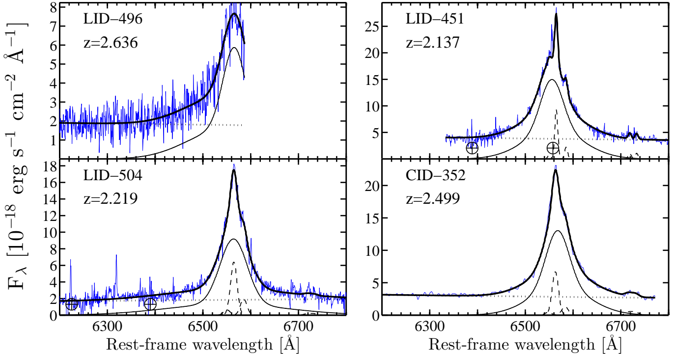
FIG. 3.— Keck/MOSFIRE spectra for the four X-ray-selected, z \simeq 2.4 COSMOS AGNs studied here (blue), along with the best-fitting spectral model (solid black lines). The data are modeled with a linear continuum (dotted), and a combination of narrow (dashed) and broad (thin solid) Gaussians. See Section 2.4 for details regarding the spectral analysis. Regions affected by telluric features are marked with encircled crosses. The spectra are shown prior to the host-light correction.
