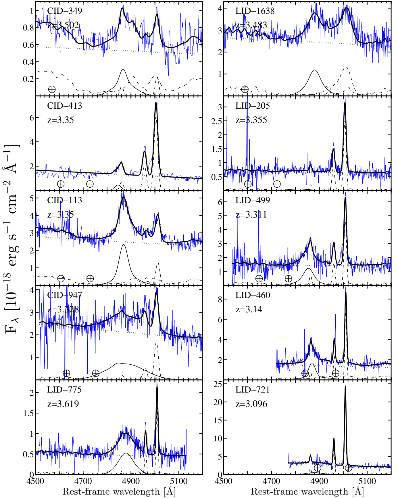
FIG. 2.— Keck/MOSFIRE spectra for the 10 X-ray-selected, z \approx 3.3 COSMOS AGNs studied here (blue), along with the best-fitting spectral model (solid black lines). The data are modeled with a linear continuum (dotted), a broadened iron template (dotted-dashed), and a combination of narrow (dashed) and broad (thin solid) Gaussians. See Section 2.4 for details regarding the spectral analysis. Regions affected by telluric features are marked with encircled crosses. The spectra are shown prior to the host-light correction. Note the near absence of broad H \beta components in objects LID-205 and LID-721, and the peculiar broad [O III] profile in LID-1638 (see Section 3.1).
