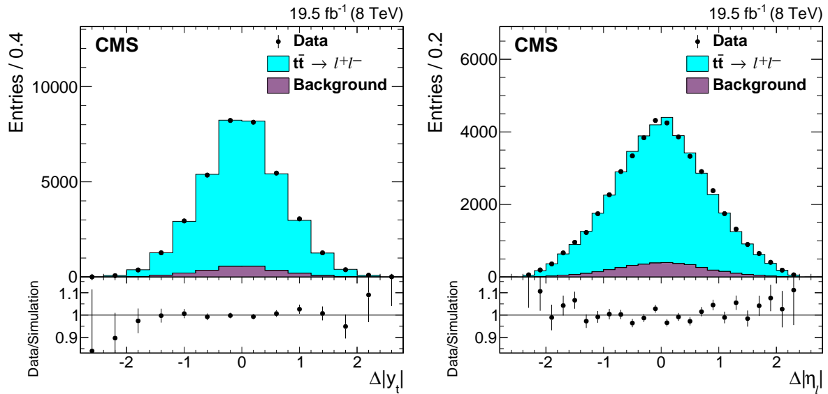
Figure A.1: Reconstructed \Delta|y_t| and \Delta|\eta_\ell| distributions from data (points) and simulation (histogram), with the predicted signal ( t\bar{t} \rightarrow \ell^+\ell^- ) and background distributions shown separately. The simulated signal yield is normalized to that of the background-subtracted data. The vertical bars on the data points represent the statistical uncertainties. The lower panels show the ratio of the numbers of events from data and simulation.
