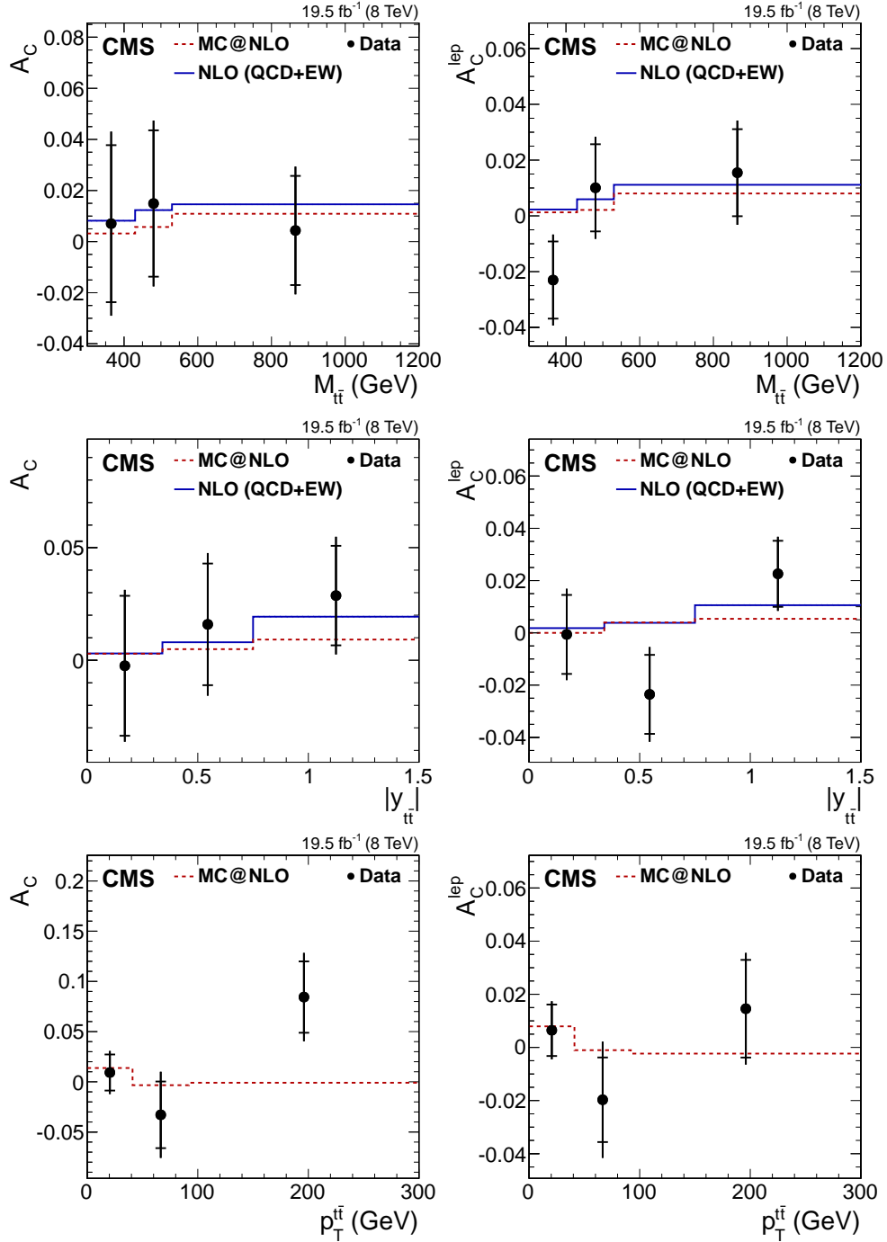
Figure 2: Dependence of the t\bar{t} and leptonic charge asymmetries A_C (left) and A_C^{\text{lep}} (right) obtained from the unfolded distributions in data (points) on M_{t\bar{t}} (upper), |y_{t\bar{t}}| (middle), and p_T^{t\bar{t}} (lower). Parton-level predictions from the MC@NLO simulation and calculations at NLO (QCD+EW) [12] are shown by dashed and solid histograms, respectively. The vertical bars show the total uncertainty, the statistical component of which is marked by a horizontal tick. The last bin of each plot includes overflow events.
