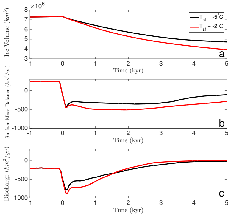
Figure 3. Sensitivity of deglacial ice sheet response to prescribed changes in sea level temperature. Black lines are configured with final T_s = -5^\circ C (same as black line in Figure 2 of main text). Red lines are configured with final T_s = -2^\circ C . (a) Ice volume. (b) Surface mass balance. (c) Discharge due to calving at the ice sheet margin following.
