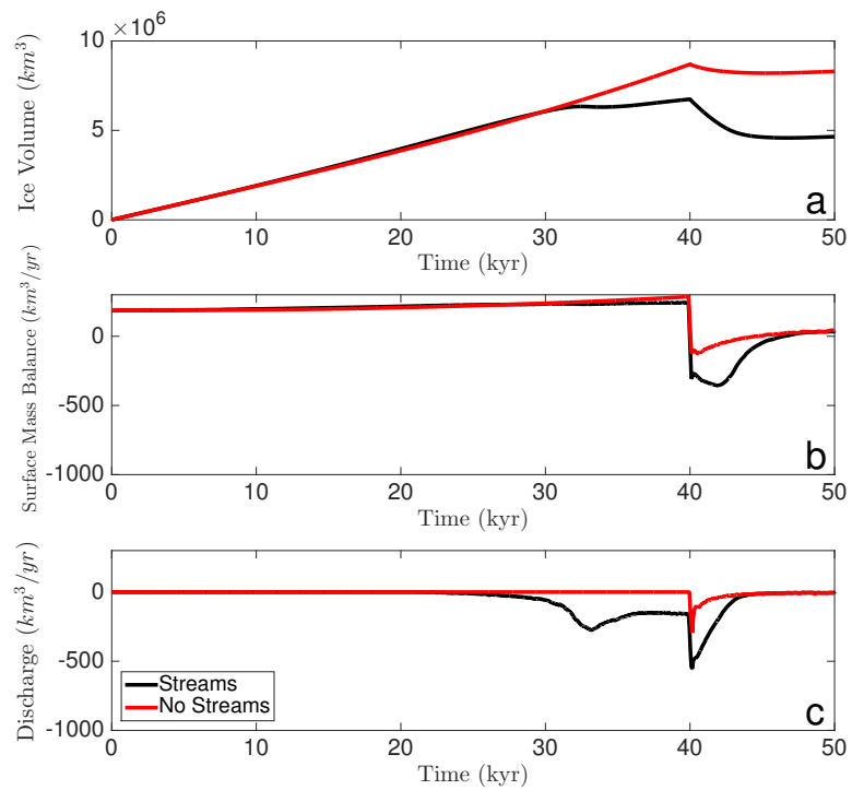
Figure 4. Sensitivity of ice sheet evolution to presence of ice streams. Black lines are configured with ice streams (same as black line in Figure 2 of main text). Red lines are configured with \phi = 80^\circ everywhere in model domain. (a) Ice volume. (b) Surface mass balance. (c) Discharge due to calving at the ice sheet margin following.
