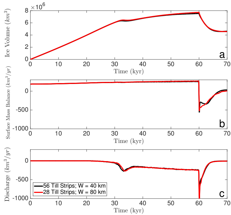
Figure 2. Sensitivity of deglacial ice sheet response to changes in till configuration. Black lines are configured with 56 weak till strips of 40 km width each (same as black line in Figure 2 of main text). Red lines are configured with 28 weak till strips of 80 km width. (a) Ice volume. (b) Surface mass balance. (c) Discharge due to calving at the ice sheet margin following.
