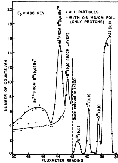
FIG. 5. Spectrometer profiles for alpha-particles, Be^{7++} ions, and scattered protons observed at \theta_{lab} = 137.8^\circ from a thin (B^{10})_2O_3 target on aluminum bombarded by 1488-kev protons.
