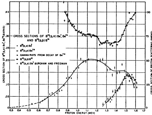
FIG. 9. Cross sections per 4\pi steradians in the center-of-mass system at \theta_{cm} \sim 140^\circ ( \theta_{lab} = 137.8^\circ ) for various B^{10} + H^1 reactions vs laboratory proton energy. The upper curve is for B^{10}(p,p)B^{10} ; the intermediate curve is for B^{10}(p,\alpha)Be^7 ; the lower curve is for B^{10}(p,\alpha')Be^{7*}(\gamma)Be^7 . The gamma-rays from the decay of Be^{7*} were measured at \theta_{lab} = 90^\circ .
