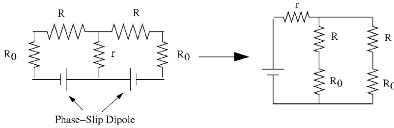
FIG. 5. Effective circuit for a phase-slip dipole with s=1 . R_Q is the effective resistance of a semi-infinite resistor ladder as given above Eq. (30). The dissipation seen by a dipole has no contribution from plasma waves at low frequencies.
