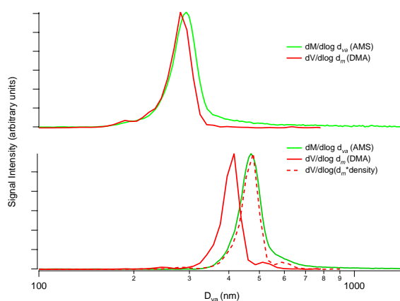
Fig. 1. Calculation of the effective density (data from exp. 14, Table 2). Panel (a) Volume distribution from the DMA ( dV/d\log(d_m) ), solid red line) and mass distribution from the cToF-AMS ( dM/d\log(d_{va}) ), solid green line) of triethylammonium nitrate (TEAN). The fact that the two distributions are aligned indicates the effective density of TEAN is \sim 1 . The slight tailing of the cToF-AMS signal could be caused by slow vaporization or higher uncertainty in the size calibration for larger particles. Panel (b) The same distributions shown in (a) after products from TEA photooxidation have condensed onto the nitrate salt shown in (a) for 7 h. The particles have grown larger from the condensation process. The dashed red line ( dV/d\log(\rho_{\text{eff}} d_m) ) is created by adjusting the effective density ( \rho_{\text{eff}} ) until the dotted red line aligns with the solid green line ( \rho_{\text{eff}} = 1.1 \text{ g cm}^{-3} ).
