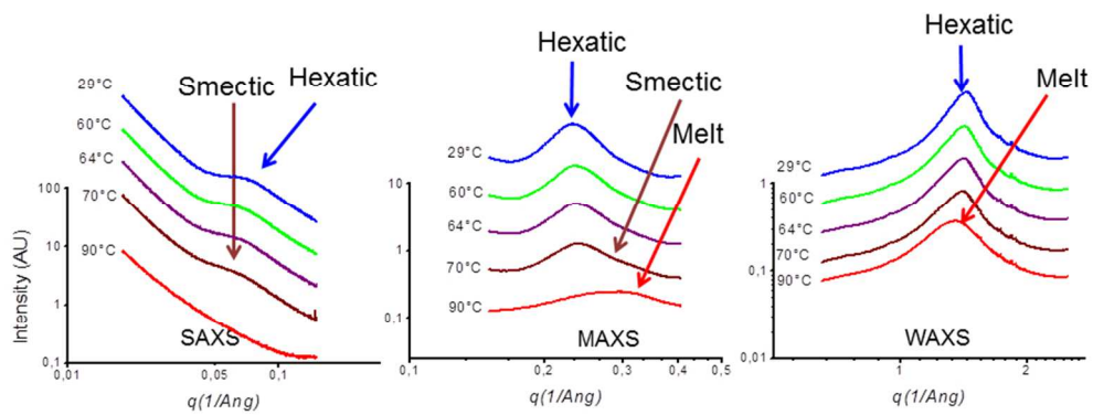
Figure S1. X-ray diffraction data from a powder sample to highlight the structural transitions. This illustrates the generality of the observation made in the main text where the data from drawn fibers are discussed.
