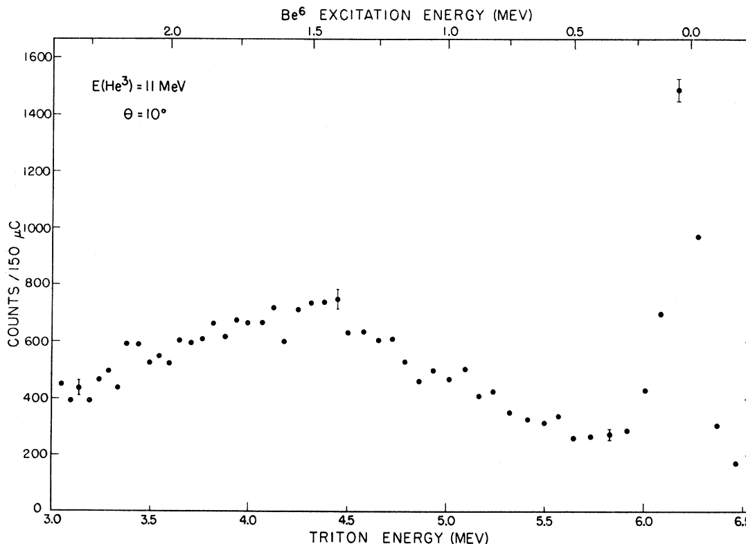
FIG. 2. Energy spectrum of tritons from \text{Li}^6 + \text{He}^3 at E_{\text{He}^3} = 11 MeV. The observation angle is 10^\circ . The experimental points were taken with a momentum window \Delta P = P/720 , and an interval P/400 between adjacent points. As presented in this figure, the yields from three adjacent counters have been summed to improve the statistics, and the yield at each value of B\rho has been divided by (B\rho)^2 in order to present an energy spectrum with constant energy interval.
