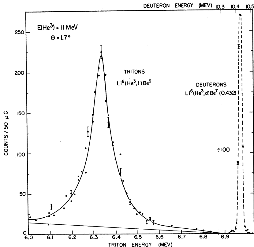
FIG. 1. Momentum spectrum of tritons and deuterons from \text{Li}^6 + \text{He}^3 at E_{\text{He}^3} = 11 MeV. The mean observation angle is 1.7^\circ . The deuteron yield has been divided by 100. The yield at each value of B\rho has been divided by B\rho to present a momentum spectrum with constant momentum interval.
