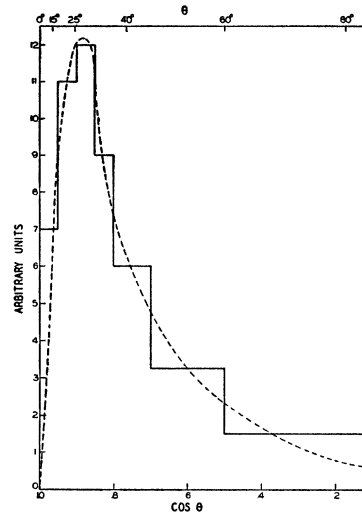
FIG. 6. Angular distribution of particles emerging from the nucleus taking into account multiple scattering (compare Fig. 3). The cosine of the laboratory scattering angle is given in the lower scale and the actual angle in the upper scale.
