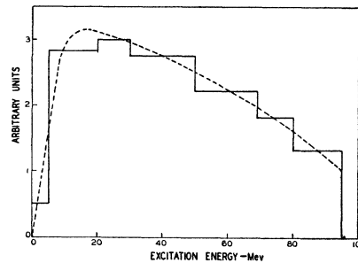
FIG. 4. Distribution of excitation energies of the residual nucleus immediately following the bombardment of a heavy nucleus by 86.6-Mev neutrons.
