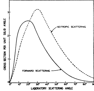
FIG. 3. Angular distribution of particles scattered by a heavy nucleus in the laboratory system assuming only a single collision inside the nucleus. The energy of the incident neutron is 90 Mev. Because of the symmetry of the neutron-proton scattering, these curves give also the distribution of recoil protons (see Section III). The ordinate scale is in arbitrary units and is not the same for the two curves.
