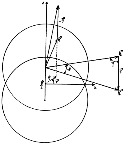
FIG. 1. Coordinate system used in computing the effective mean free path and the angular distribution of scattered particles.
