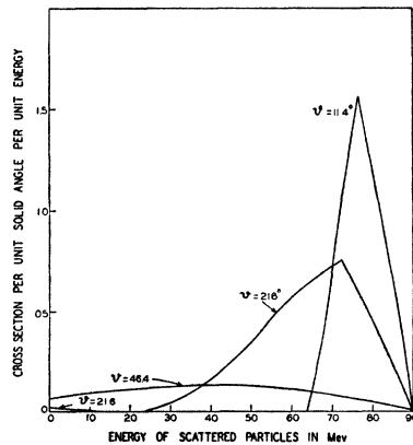
FIG. 2. Energy distribution of particles scattered from a heavy nucleus at fixed laboratory scattering angles. The energy of the incident neutron is 90 Mev. The discontinuous derivatives at the maxima result from the exclusion principle. The ordinate scale is in arbitrary units.
