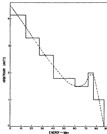
FIG. 5. Energy distribution of particles emerging at all angles immediately after the bombardment of a heavy nucleus by 86.6-Mev neutrons.
