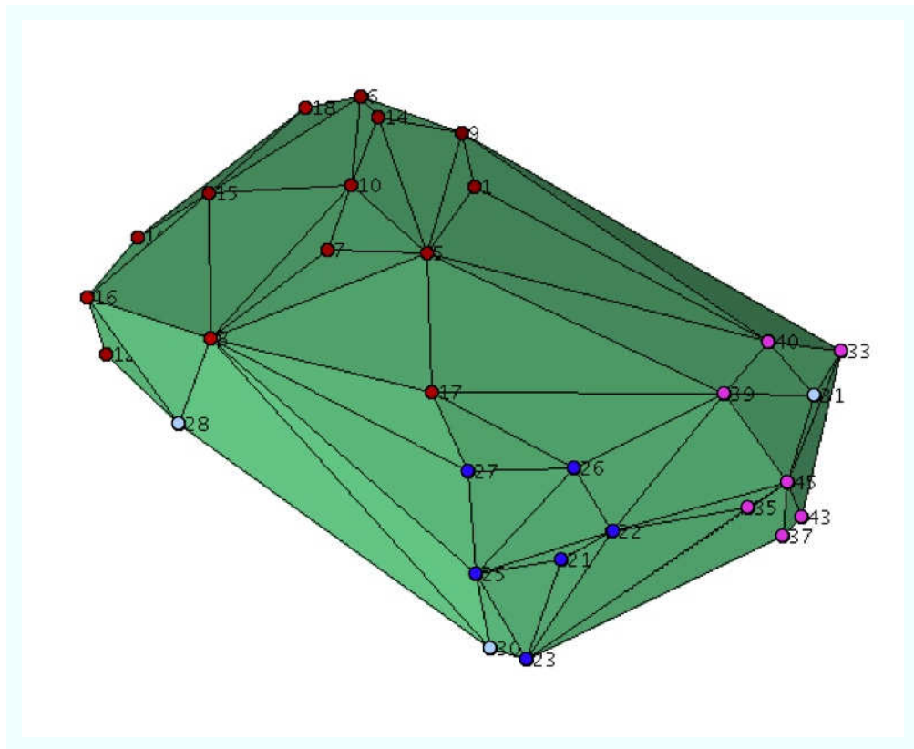
Figure 2: The 3-dimensional PCA projection of the ENr131 ENCODE genotype. The colors of the vertices represent the different populations: red=CEU, blue=CHB, cyan=JPT, pink=YRI.
