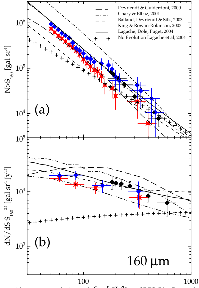
FIG. 3.— Source counts at 160 \mu\text{m} with no correction for incompleteness. Star: CDFS; Blue Diamond: Marano field; Black Diamond: ISO FIRBACK 170 \mu\text{m} counts from Dole et al. (2001). Top panel (a): Integral Source counts. For clarity, photometric uncertainty is only shown for S_{160} > 200 \text{ mJy} . Lower panel (b): Differential Source counts. Models are also plotted with the same symbols as Figure 2.
