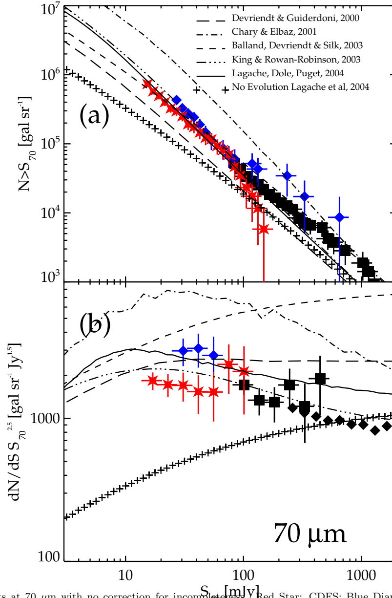
FIG. 2.— Source Counts at 70 \mu\text{m} with no correction for incompleteness. Red Star: CDFS; Blue Diamond: Marano; Black Square: Boötes Field; Black Diamond: IRAS 60 \mu\text{m} counts from Lonsdale et al. (1990) converted at 70 \mu\text{m} . Top panel (a): Integral Source Counts. For clarity, photometric uncertainty is only shown for S_{70} > 100 \text{ mJy} . Bottom panel (b): Differential Source Counts. Models are also plotted: long dash: Devriendt & Guiderdoni (2000); dash-dot: Chary & Elbaz (2001); dash: Balland et al. (2003); dash-dot-dot-dot: King & Rowan-Robinson (2003); solid line: Lagache et al. (2004); plus: No Evolution Model.
