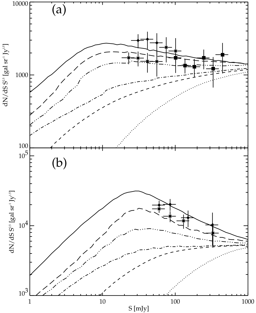
FIG. 4.— Cumulative contributions to the Differential Source Counts at 70 \mu\text{m} and 160 \mu\text{m} of galaxies, as a function of redshift, from the model of Lagache et al. (2004). Top panel (a): 70 \mu\text{m} . Bottom panel (b): 160 \mu\text{m} . Symbols are described in Figures 2 and 3. Galaxies contributing to the counts at Redshifts 0.1 (dot), 0.3 (dash), 0.7 (dot-dash), 0.9 (dot-dot-dot-dash) and 1.1 (long dash). The total contribution is the upper solid line.
