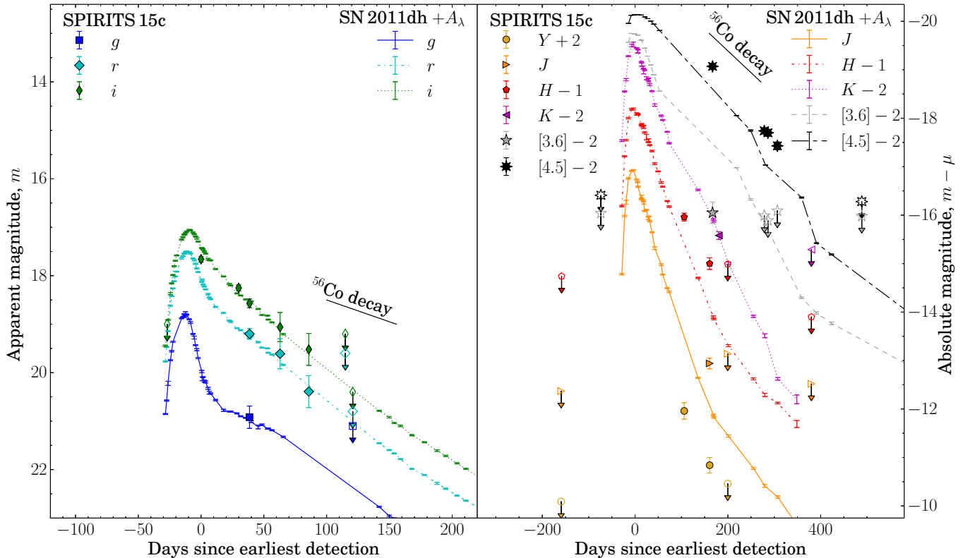
Figure 2. The optical ( gri ; AB magnitudes; left panel), and IR ( YJHK , [3.6], and [4.5]; Vega magnitudes; right panel) light curves of SPIRITS 15c (points) and the Type IIb SN 2011dh (lines). Unfilled points with downward arrows indicate upper limits. Error bars are shown but are sometimes smaller than the points. Time on the x -axis is given as the number of days since the earliest detection of SPIRITS 15c on 2014 August 21.4 (MJD = 56890.4). The light curves of SN 2011dh are shifted in apparent magnitude to the distance of SPIRITS 15c, with applied total reddening characterized by E(B - V)_{\text{MW}} + E(B - V)_{\text{host}} = 0.72 mag, or A_V \approx 2.2 magnitudes of extinction assuming a standard R_V = 3.1 extinction law (Fitzpatrick 1999; Chapman et al. 2009; Schlafly & Finkbeiner 2011). The phase of the SN 2011dh light curves is set so that the earliest detection of SN 2011dh coincides with the most constraining non-detection preceding the outburst of SPIRITS 15c. For comparison, we also show the expected decay rate for a light curve powered by the radioactive decay of ^{56}\text{Co} (see Gehrz 1988; Gehrz & Ney 1990).
