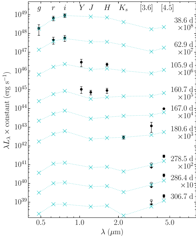
Figure 7. Comparison of the SED evolution of SPIRITS 15c (black circles) and SN 2011dh (cyan ‘X’-symbols). Unfilled points with downward arrows represent upper-limits. The band-luminosities for SPIRITS 15c are corrected for Galactic extinction to IC 2163 from NED (Fitzpatrick 1999; Schlafly & Finkbeiner 2011; Chapman et al. 2009). The points for are SN 2011dh drawn from a linear interpolation of the SN 2011dh light curves, and reddened by the assumed excess extinction in SPIRITS 15c characterized by E(B - V)_{\text{host}} = 0.65 with a standard R_V = 3.1 extinction law. Error bars for SPIRITS 15c are shown, but are sometimes smaller than the plotting symbols. The phase, set as in Figure 2, of each SED is listed along the right side, and each SED is shifted up by a factor of 10 from the one below for clarity.
