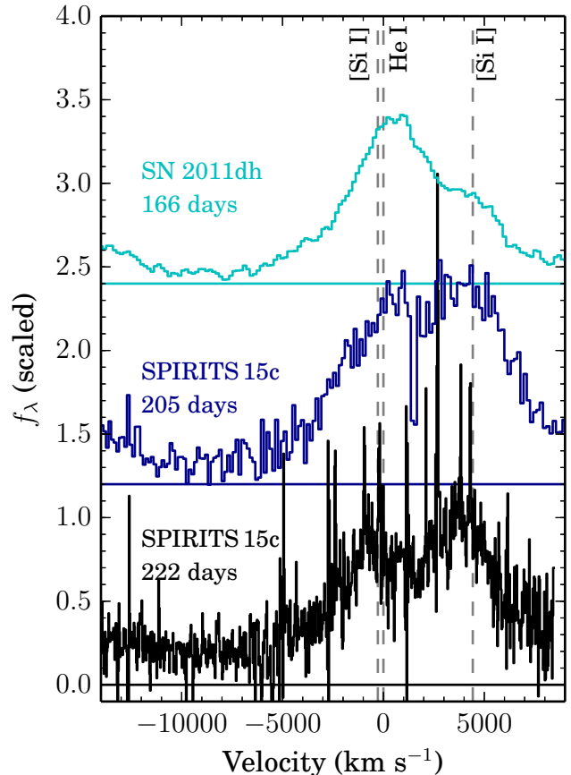
Figure 6. The observed velocity profile of the He I line at 1.0830 \mu\text{m} in the spectra of SN 2011dh at a phase of 166 days (top) and SPIRITS 15c at phases of 205 (middle) and 222 days (bottom). The phase of the SN 2011dh spectrum is set as in Figure 2. The profiles are scaled and shifted arbitrarily in flux for clarity.
