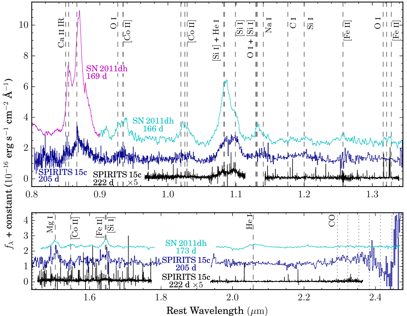
Figure 4. The NIR spectra of SPIRITS 15c taken with Baade/FIRE on t = 205 days (blue) and Keck/MOSFIRE on t = 222 days (black) shifted to the rest frame of the the location of SPIRITS 15c measured in an ALMA CO velocity map of IC 2163 ( v_{\text{CO, helio}} = 2827 \text{ km s}^{-1} , Elmegreen et al. 2016). The Keck/MOSFIRE spectrum is multiplied by a factor of 5 and the Baade/FIRE spectrum is shifted up by 10^{-16} \text{ erg s}^{-1} \text{ cm}^{-2} \text{ \AA}^{-1} for clarity. We also show late-time spectra of SN 2011dh for comparison (cyan and magenta), shifted up by 2 \times 10^{-16} \text{ erg s}^{-1} \text{ cm}^{-2} \text{ \AA}^{-1} , where the phases marked on the plot are set as in Figure 2. Dashed vertical lines show the locations of atomic transitions identified in the spectra of SN 2011dh by Ergon et al. (2014, 2015) and Jerkstrand et al. (2015). Dotted vertical lines mark the band heads of the \Delta v = 2 vibrational overtones of ^{12}\text{C}^{16}\text{O} , which may contribute to excess flux observed between 2.3 and 2.5 \mu\text{m} .
