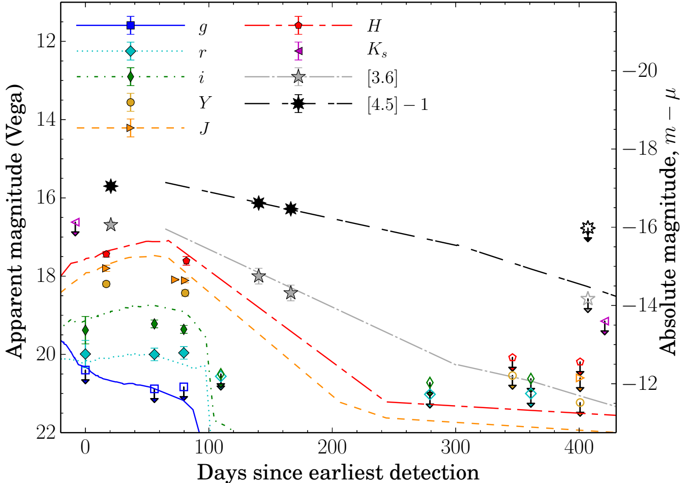
Figure 3. The optical ( gri ; AB magnitudes), and IR ( YJH , [3.6], and [4.5]; Vega magnitudes) light curves of SPIRITS 14buu (points). Also shown are the griJH light curves of the Type IIP SN 2005cs and the [3.6] and [4.5] light curves of SN 2004et (lines). Unfilled points with downward arrows indicate upper limits. Error bars are shown, but are usually smaller than the points. Time on the x -axis is given as the number of days since the earliest detection of SPIRITS 14buu on MJD = 56650.3. The light curves of SN 2005cs are shifted in absolute magnitude by 0.1 mag, with applied total reddening characterized by E(B - V) = 0.49 , or A_V \approx 1.5 mag assuming a standard R_V = 3.1 extinction law (Fitzpatrick 1999; Chapman et al. 2009; Schlafly & Finkbeiner 2011). The light curves of SN 2004et are shifted fainter by 2.4 mag. The phase of the SN 2005cs light curves is set so that fall-off of the plateau lines up with that of SPIRITS 14buu. The phase of the SN 2004et light curves is time in days from the assumed explosion epoch (MJD = 53270.0; Li et al. 2005).
