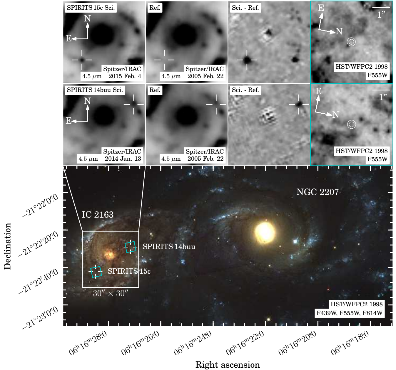
Figure 1. The bottom panel shows color-composite, archival HST /WFPC2 imaging of the interacting galaxy pair of IC 2163 and NGC 2207 from 1998 in three filters (F439W in blue, F555W in green, and F814W in red). The positions of SPIRITS 15c and SPIRITS 14buu in dusty spiral arms of IC 2163 are indicated with the crosshairs. The right panels of the top and middle rows show zoom-ins of the F555W image to the regions indicated by the cyan squares for SPIRITS 15c and SPIRITS 14buu, respectively. The white circles show the 3- and 5- \sigma uncertainties on the position of transients. We are unable to identify an individual star as a candidate progenitor in either case. The left three panels in the top and middle rows show the 30'' \times 30'' region indicated by the white zoom-in box. The first panels from the left are the Spitzer /IRAC discovery science frames at [4.5] from 2015 February 4.4 (top row; SPIRITS 15c) and 2014 January 13.9 (middle row; SPIRITS 14buu), the second are the reference images from 2005 February 22.7 (PID3544; PI D. M. Elmegreen), and the third are the science – reference subtraction images, clearly showing the new, transient sources. We note in the SPIRITS 15c discovery and subtraction images that the apparent variability of the galaxy nucleus and the apparent new source directly to the west of SPIRITS 15c are likely spurious.
