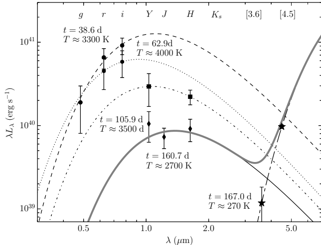
Figure 5. The optical to IR SED of SPIRITS 15c at multiple epochs during the evolution of the transient. Band-luminosities ( \lambda L_\lambda ), calculated assuming a distance to IC 2163 of 35.5 Mpc and correcting for Galactic reddening characterized by E(B - V) = 0.072 mag, are shown at t = 38.6 (circles), 62.9 (hexagons), 105.9 (squares), 160.7 (diamonds), and 167.0 days (stars). Best-fit, single-component blackbody curves are shown as black dashed, dotted, dash-dotted, solid, and long-short dashed lines, respectively, with their corresponding temperatures labeled. Since the final two epochs are nearly contemporaneous ( \Delta t = 6.3 days), we show the sum of these two blackbody components as the solid gray curve.
