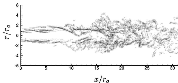
Fig. 2 Contours of the instantaneous T_{ij,ij} in the plane \theta = 0, \pi : 10 evenly spaced contours between \pm 5\rho_j U_j^2/r_0^2 .
