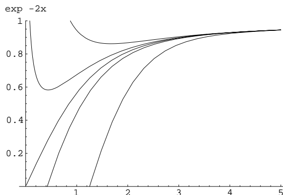
Figure 1: The function e^{-2x(\rho)} vanishes at some \rho_0 > 0 for c_0 < 0 . The figure shows the different curves for the values c_0 = -6, -0.5, 0, 0.4, 1.2 .
