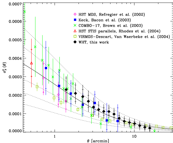
Figure 8. Shear variance in (circular, top-hat) cells, as a function of the radius of the cells. Our results are compared to those from similarly deep surveys by other groups. For ease of comparison, all results have been rescaled as if their median source redshift had been the same (see text). As in figure 3, the theoretical curves are predictions for a \Lambda CDM cosmology, with \Omega_m = 0.3 , \Omega_\Lambda = 0.7 , \Gamma = 0.21 and \sigma_8 ranging from 0.7 (bottom) to 1.2 (top).
