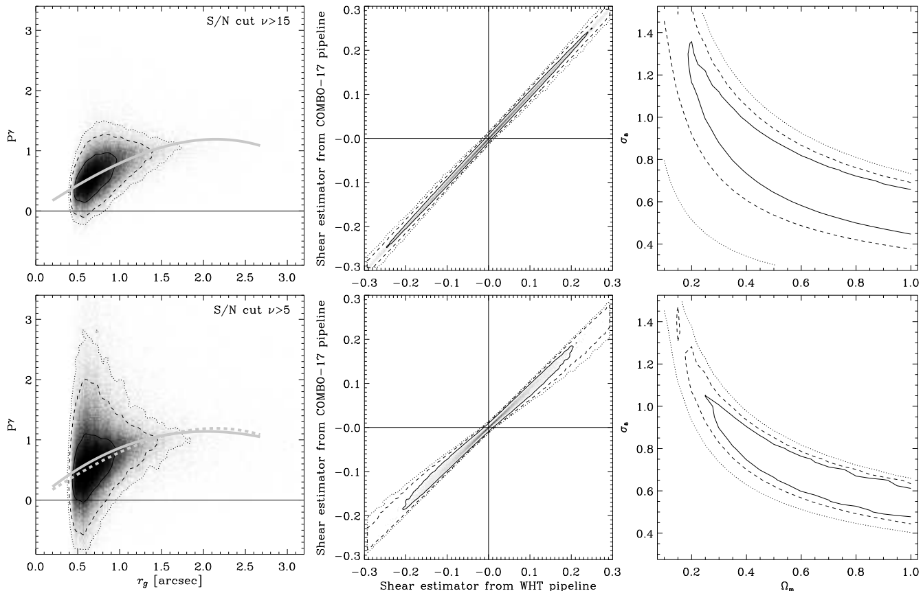
Figure 13. Left panels: The shear susceptibility factor P^\gamma for all galaxies, as a function of their size r_g , with different options for the signal-to-noise cut in the catalogue. The greyscale shows the number density of galaxies throughout the parameter space, calculated by the COMBO-17 pipeline. The WHT pipeline produces results almost identical to the top-left panel. In practice the fit is performed on galaxies for one image at a time, and is therefore more noisy; the fit to all galaxies here is shown merely to guide the eye. The fit in the bottom panel is reproduced as a dashed line in the bottom panel. When the COMBO-17 pipeline uses a signal to noise cut of \nu > 5 , the population ensemble’s average shear susceptibility is raised. Middle panels: A comparison of the shear estimators derived via the WHT and the COMBO-17 shear measurement pipelines. Only subsequently matched galaxies are included in this plot, and the WHT pipeline always uses a signal to noise cut to the catalogue of \nu > 15 , so all galaxies shown are brighter than that. Consistent results are obtained in the top panel, where the COMBO-17 pipeline also uses a cut of \nu > 15 . The unbiased, 1% dispersion of individual values is merely due to the different interpolation of the PSF across individual fields. When the COMBO-17 pipeline uses a signal to noise cut of \nu > 5 , the shear estimators of all galaxies are lowered, including these bright ones. Right panels: Constraints upon cosmological parameters \Omega_m and \sigma_8 , from a maximum-likelihood analysis of shears measured with the COMBO-17 pipeline, using different options for the signal-to-noise cut. The 68.3%, 95.4% and 99.7% confidence contours are shown.
