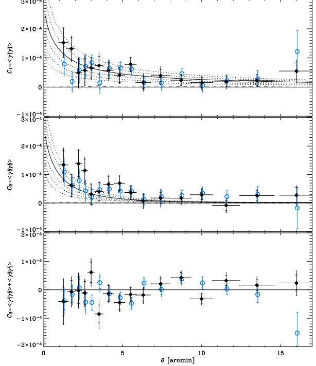
Figure 3. Correlation functions of the shear field measured in our 4 square degree WHT survey. The solid data points show our measurement. The inner error bars are for statistical errors only; the outer error bars also include full non-Gaussian sample variance. The blue circles show measurements of our data by the COMBO-17 pipeline, artificially adjusted to correct for its slightly higher source redshift distribution and permit easy comparison. The solid line shows the theoretical prediction for a \Lambda CDM model with \Omega_m = 0.3 , \Omega_\Lambda = 0.7 , \Gamma = 0.21 and \sigma_8 = 1.0 , assuming a median source redshift of z_s = 0.8 and using the fitting functions of Smith et al. (2003). The dotted lines show similar theoretical predictions, but with \sigma_8 ranging from 0.7 (bottom) to 1.2 (top). The dashed lines barely visible above the x axis show the correlation of galaxy shears with the observed PSF anisotropy.
