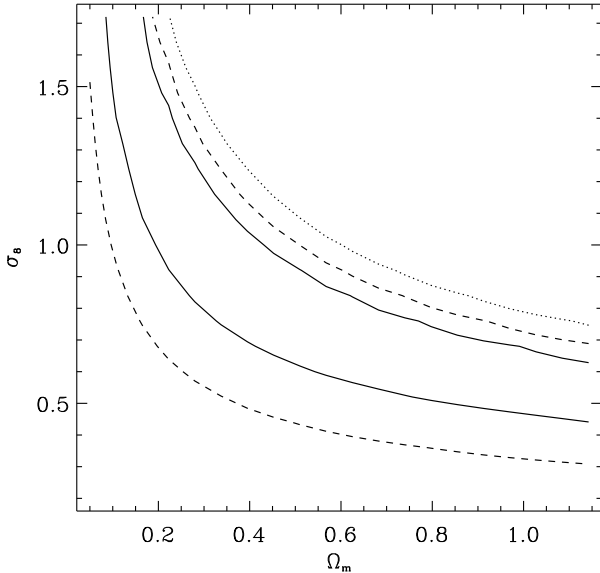
Figure 6. Constraints upon cosmological parameters from the Keck cosmic shear survey by Bacon et al. (2003), showing the 68.3%, 95.4% and 99.7% confidence limits as in figure 5. Only one edge of the 99.7% confidence contour is visible inside this parameter range.
