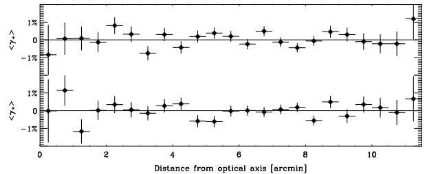
Figure 12. The radial and “curl” components of galaxy shears as a function of distance from the field centre/optical axis, averaged over all the fields used in our survey. That this is consistent with zero on all scales demonstrates an absence of systematics concerning alt-az tracking, and the successful correction of astrometric distortions within the telescope, whose expected behaviour is purely radial (see §2).
