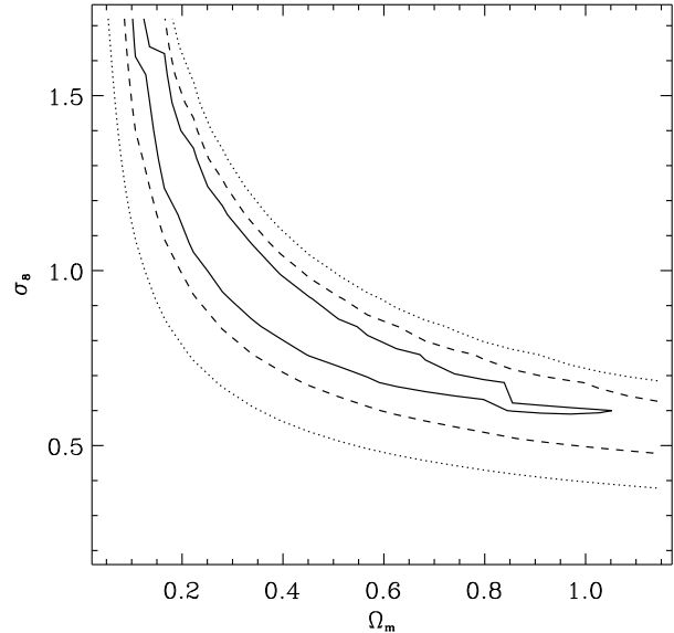
Figure 7. Constraints upon cosmological parameters for the combination of both WHT and Keck surveys, showing the 68.3%, 95.4% and 99.7% confidence limits, as in figure 5.
