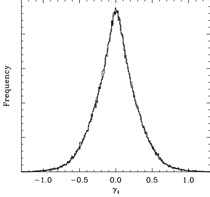
Figure 2. The distribution of measured shear estimators from all galaxies used in the WHT survey. A fitting function is given in the text. The two components of shear are shown superimposed; their distributions are indistinguishable. Notice, however, the extended wings typical of the KSB method.
