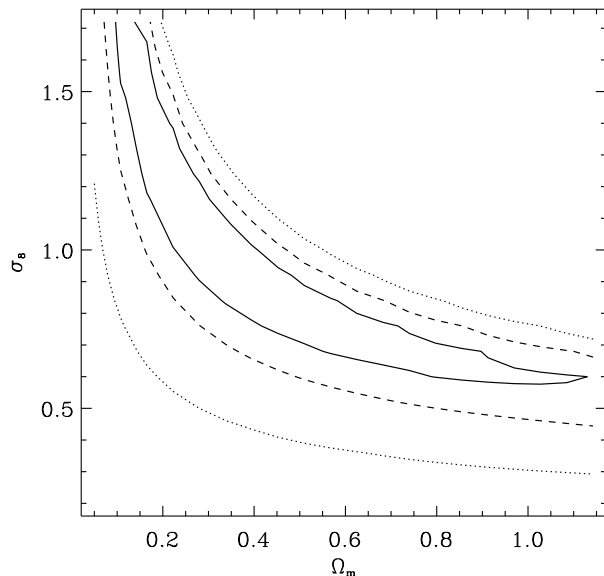
Figure 5. Constraints upon cosmological parameters \Omega_m and \sigma_8 , from a maximum-likelihood analysis of our WHT cosmic shear survey data. The 68.3% (solid), 95.4% (dashed) and 99.7% (dotted) confidence limits include statistical errors and non-Gaussian cosmic variance. However, they include neither the calibration of the shear measurement method, nor uncertainty in the source galaxy redshift distribution. These sources of error are considered separately in the text.
