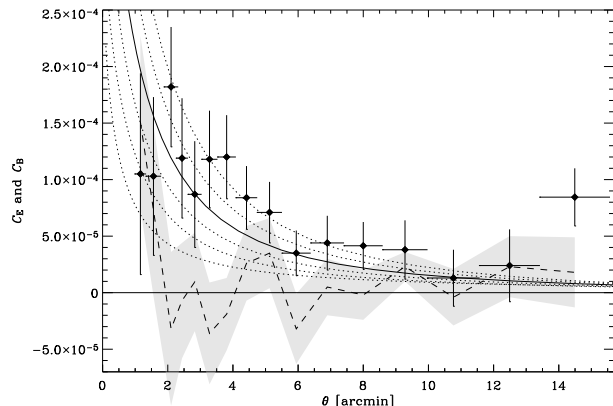
Figure 9. E - B decomposition of the shear field observed in our WHT survey. The points show the measured E (tangential) modes of the shear field. As in figure 3, the theoretical curves are predictions for a \Lambda CDM cosmology, with \Omega_m = 0.3 , \Omega_\Lambda = 0.7 , \Gamma = 0.21 and \sigma_8 ranging from 0.7 (bottom) to 1.2 (top). The dashed line shows our measured B -mode (curl) signal, and the shaded region shows its 1\sigma error bar. In the absence of systematics, the B -mode should be consistent with zero.
