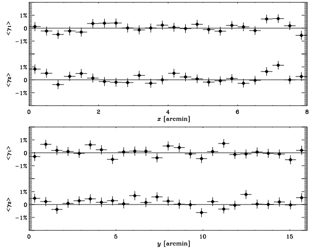
Figure 11. Galaxy shears as a function of position on the WHT CCD, averaged over all the fields used in our survey. That this is consistent with zero everywhere demonstrates an absence of systematics concerning CCD readout, telescope vibration and tracking.
