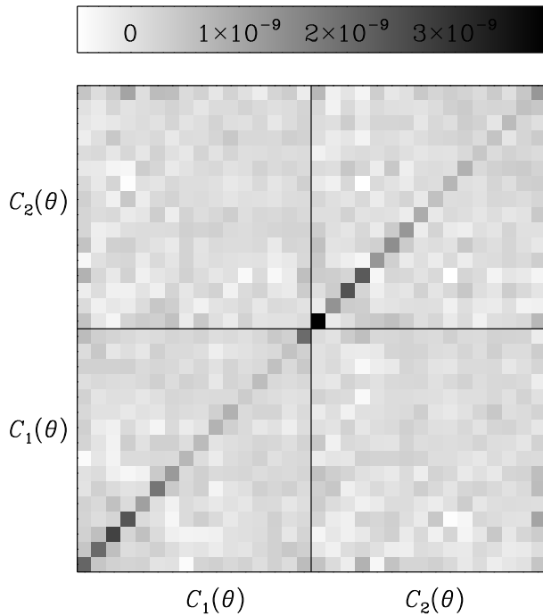
Figure 4. Covariance matrix of different angular bins of the shear correlation functions shown in figure 3, from small to large \theta , then from small to large \theta again. For example, the bottom-left quarter shows \text{cov}[C_1(\theta), C_1(\vartheta)] . The diagonal elements within this are the variances in each bin.
