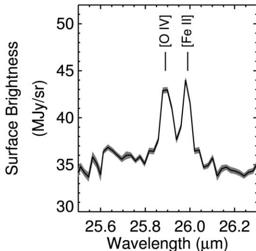
FIG. 4.—High-resolution IRS spectrum of the nucleus in NGC 4594 at 25.5–26.5 \mu\text{m} . The gray regions around the lines represent the uncertainties in the spectra. This plot shows the detail in the [O IV] and [Fe II] line emission.
