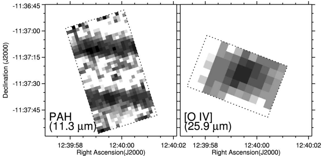
FIG. 5.—Images of the 11.3 \mu\text{m} PAH feature (left) and the 25.9 \mu\text{m} [O IV] line (right) for the inner 75'' of NGC 4594. These are images made from the IRS spectral cubes. The dotted lines show the regions covered by the IRS observations. The continuum has been identified and subtracted from the two wave bands on a pixel-by-pixel basis. Note that the PAH emission originates primarily from the ring, whereas the [O IV] emission originates primarily from the nucleus. [See the electronic edition of the Journal for a color version of this figure.]
