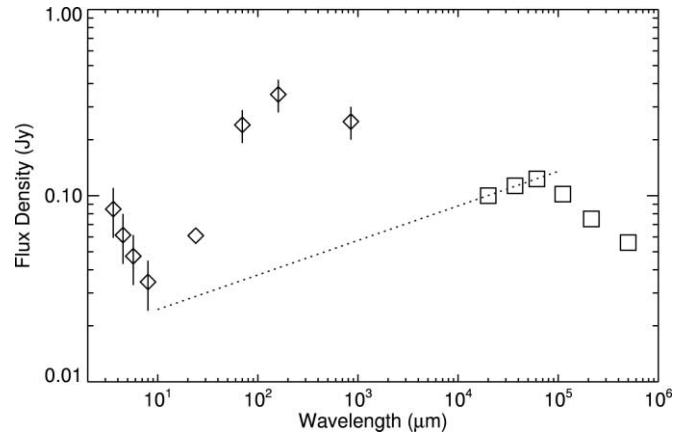
FIG. 9.—Observed SED of the AGN of NGC 4594 (diamonds), along with the radio observations by Hummel et al. (1984; squares) and the power law for the synchrotron emission as inferred from the radio data (dotted line). Except where shown, the error bars are equal to or smaller than the size of the plot symbols. Note that the extrapolations fall short of the measured 850 \mu\text{m} flux density. See the text for a discussion of radio observations other than those in Hummel et al. (1984).
