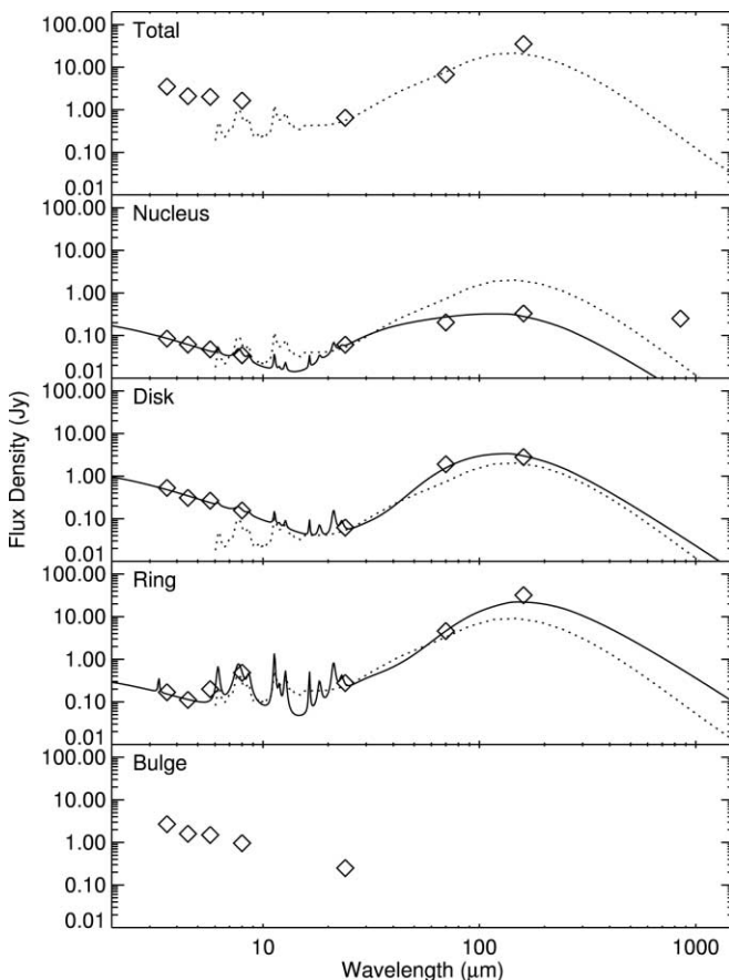
FIG. 8.—SEDs of the separate components of NGC 4594. The error bars are equal to or smaller than the size of the plot symbols. For comparison between the SEDs, the y-axes of all the plots are fixed to the same scale. For comparison to the SEDs of nearby galaxies, the semiempirical dust model from Dale et al. (2005) with a median \alpha -value (explained in the text) is plotted over the total, nucleus, disk, and ring SEDs as a dotted line. This semiempirical model has been scaled to match the 24 \mu\text{m} flux density in each SED. Emission models comprised of starlight added to the Li & Draine (2001) dust models are included in the plots of the nucleus, disk, and ring SEDs.
