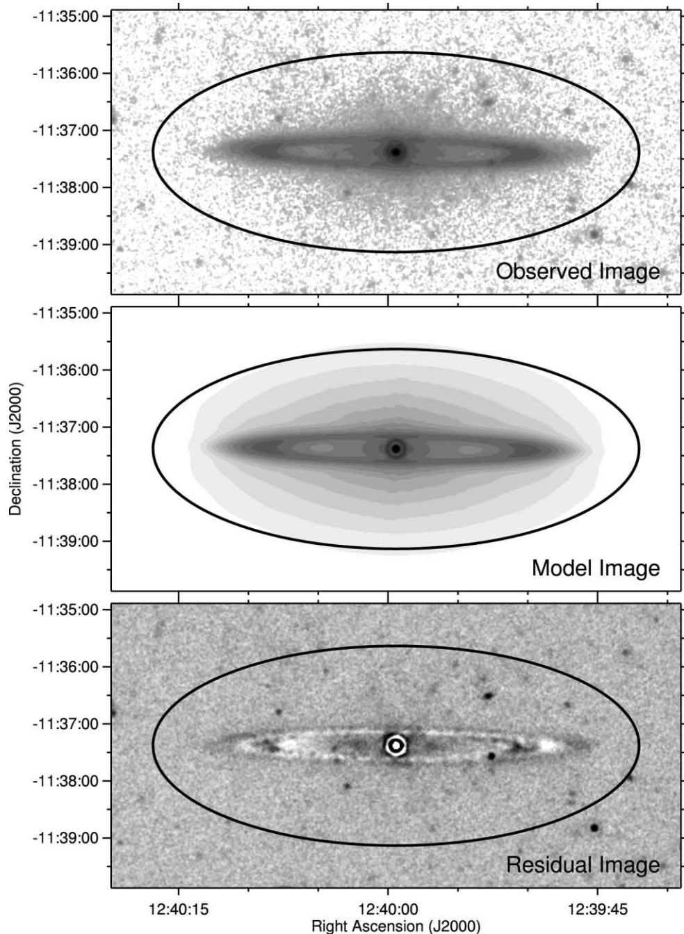
FIG. 7.—Observed 24\ \mu\text{m} image, the model 24\ \mu\text{m} image, and the residuals from subtracting the model from the observed image. This is presented as an example of the image models that were fit to the data. The optical disk of the galaxy (as given by de Vaucouleurs et al. 1991) is overplotted as ovals to show the region over which the fit was performed. [See the electronic edition of the Journal for a color version of this figure.]
