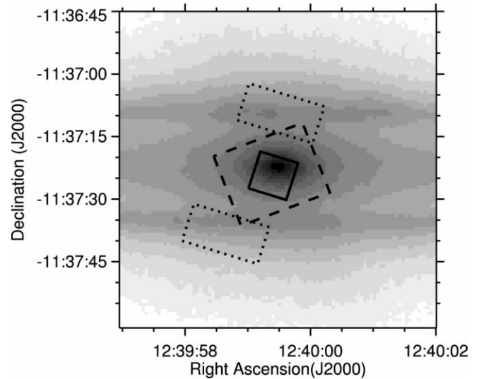
FIG. 2.—Image of the central 75'' of NGC 4594 at 8 \mu\text{m} , with boxes showing the regions in which mid-infrared spectra were extracted. The square with the solid line in the center shows where the low-resolution 5 – 38 \mu\text{m} spectrum for the nucleus was extracted. The dotted rectangles at top and bottom show where the low-resolution 5 – 38 \mu\text{m} spectrum for the ring was extracted. The dashed rectangle in the center shows where the high-resolution 25 – 27 \mu\text{m} spectrum for the nucleus was extracted. [See the electronic edition of the Journal for a color version of this figure.]
