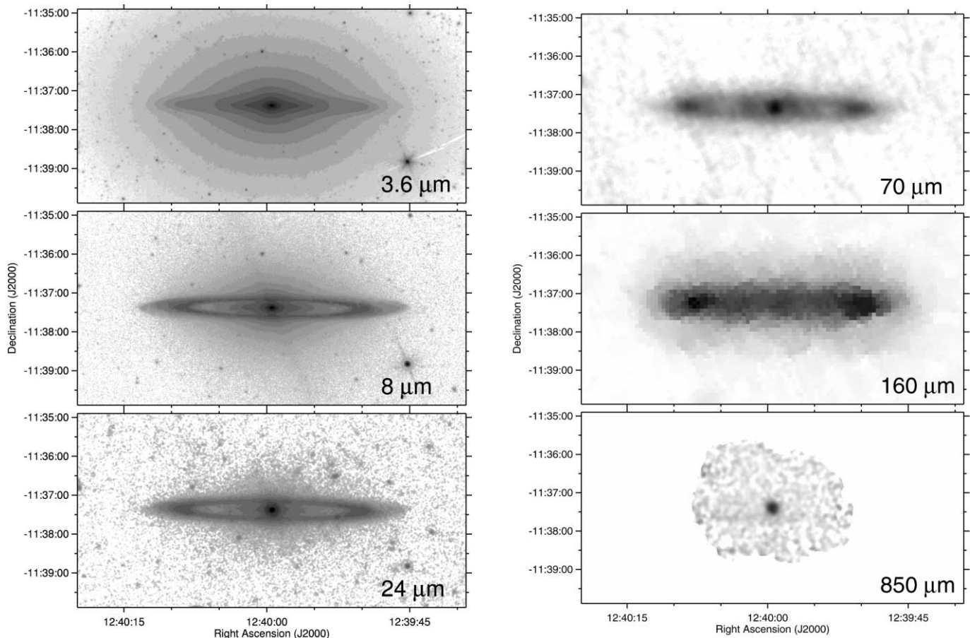
FIG. 1.—Images of NGC 4594 at 3.6, 8, 24, 70, 160, and 850 \mu\text{m} . Each image is 10' \times 5' , with north up and east to the left. The scaling of the brightness in all images is logarithmic. Note that only the inner \sim 3' \times \sim 2'.25 region was covered in the 850 \mu\text{m} band and that the very bright and dark pixels at the edges of this region are an artifact of the data processing. [See the electronic edition of the Journal for a color version of this figure.]
