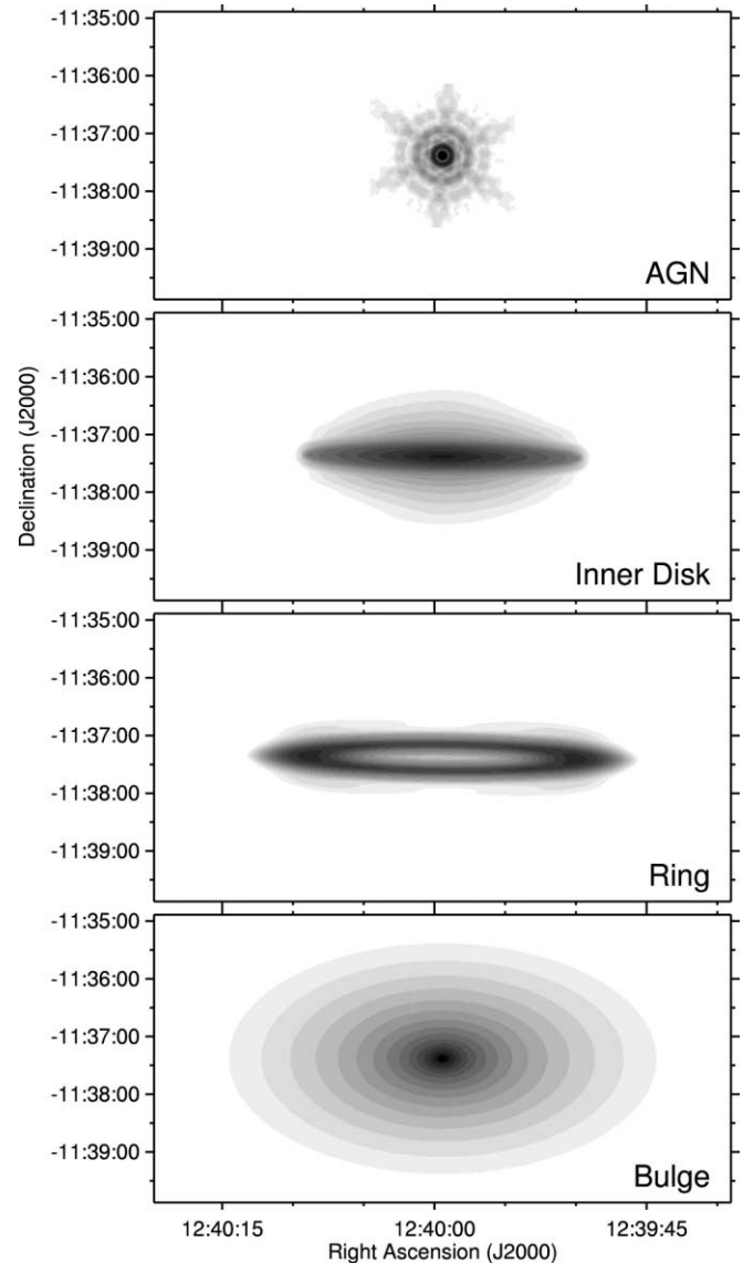
FIG. 6.—Models of the AGN, inner disk, ring, and bulge (all convolved with the 24 \mu\text{m} model PSF) made using the parameters determined from fitting the models to the 24 \mu\text{m} image. This is presented as an example of the image models that were fit to the data. For display purposes, the brightnesses of the model components are not scaled relative to each other. [See the electronic edition of the Journal for a color version of this figure.]
