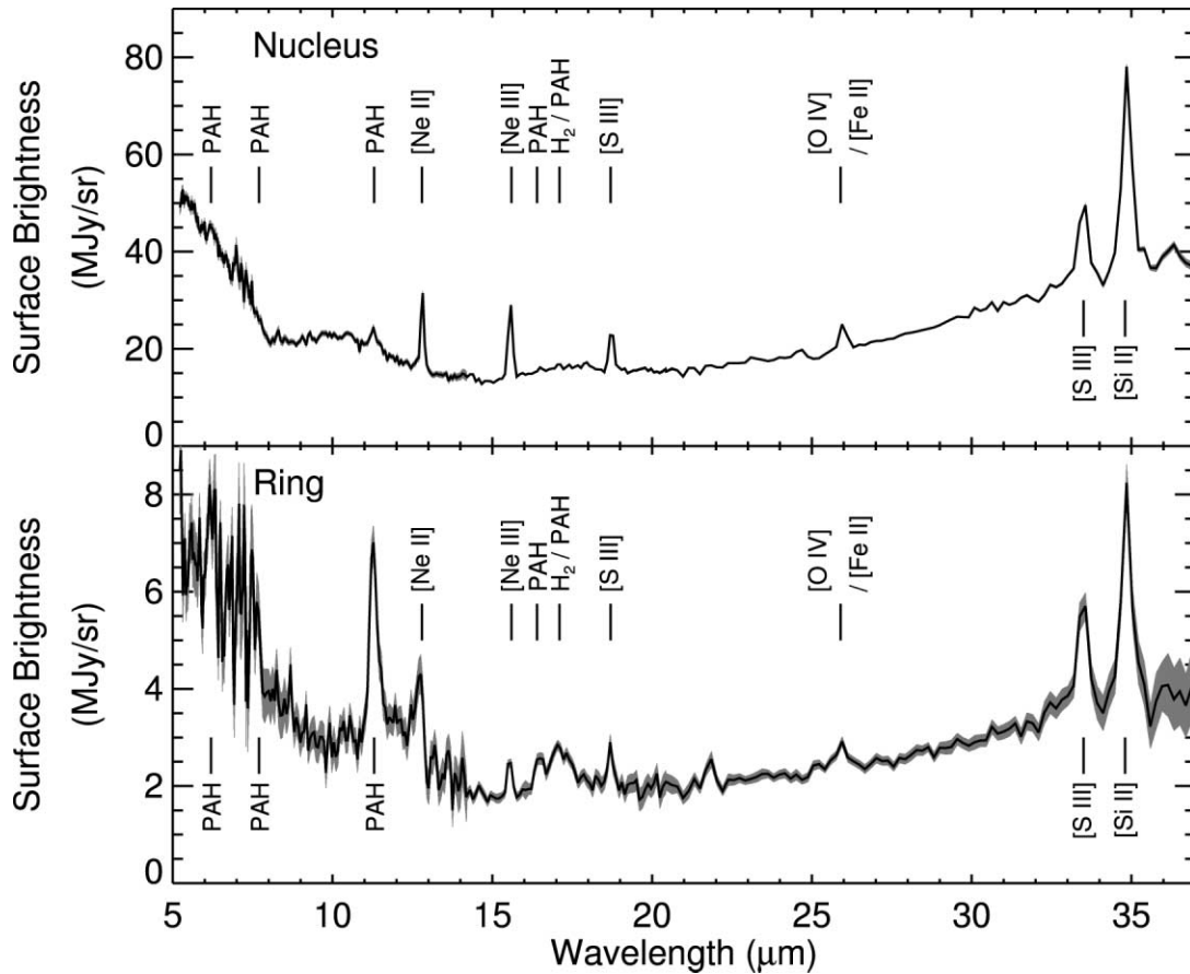
FIG. 3.—Low-resolution IRS spectra of the nucleus and the ring in NGC 4594 at 5–38 \mu\text{m} . The gray regions around the lines represent the uncertainties in the spectra. Major spectral features are identified in the plot. Note the weak or absent PAH features in the nucleus, in contrast to the strong PAH features in the ring. Because of the limitations of the spatial resolution of the telescope, the spectral features longward of 20 \mu\text{m} in the ring spectrum probably include emission from the center. See the text for additional details. See Fig. 4 to see a higher resolution 25.5–26.5 \mu\text{m} spectrum of the nucleus in which the [O IV] and [Fe II] lines are separated.
