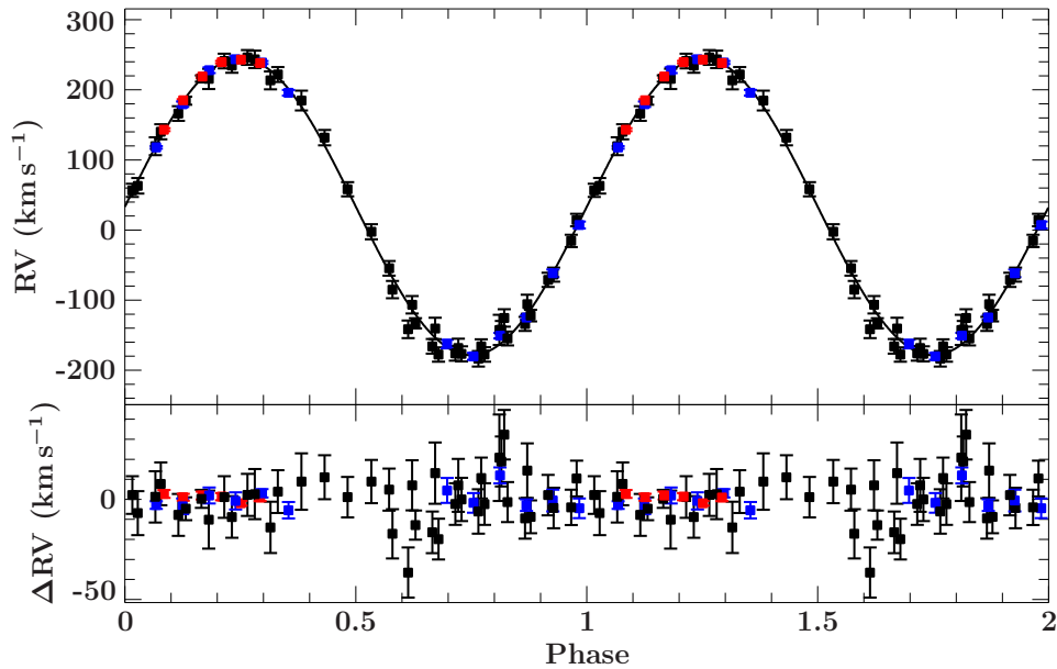
Figure 3. Radial velocity curve of PTF1 J082340.04+081936.5. For details see Kupfer et al. (2016).
