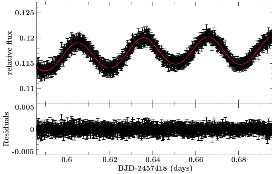
Figure 2. Light curve of PTF1 J082340.04+081936.5 shown with a model fit For details see Kupfer et al. (2016).
