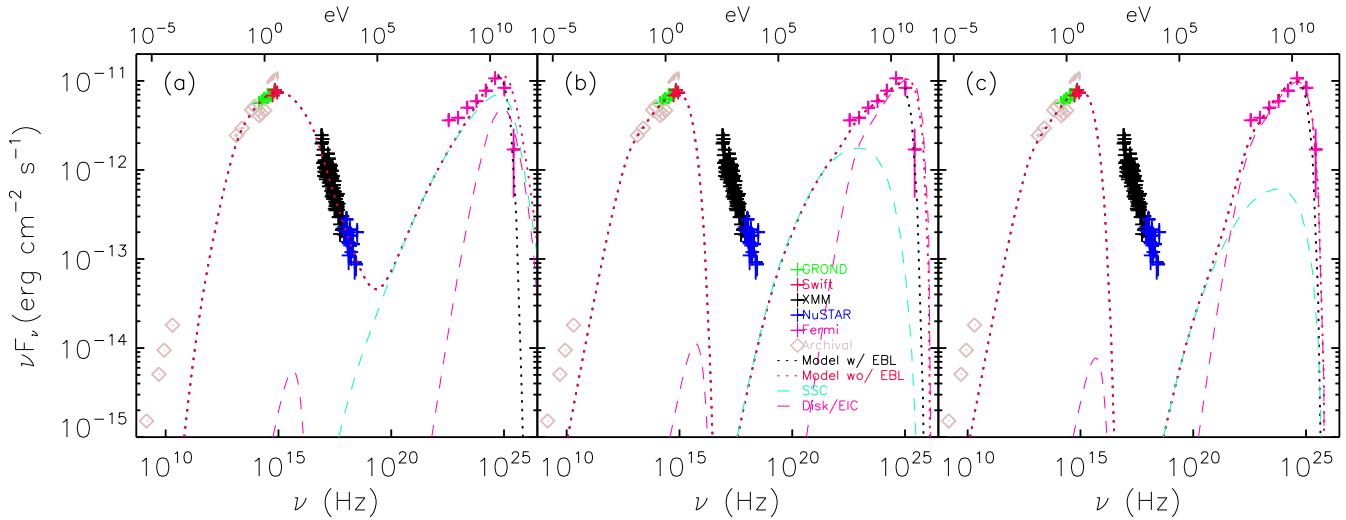
Figure 5. SED models with the disk component for J0630. (a): A model with the disk component added to the baseline synchrotron+SSC model in Figure 3b. (b): Similar to (a), but baseline model is that in Figure 4. (c): Same as (b) with larger B and lower \gamma'_{\max} . The model parameters are further adjusted from the baseline ones to match the SED. The EBL model we used for the plot is the “Finke C” model in Table 4. See text for more details.
