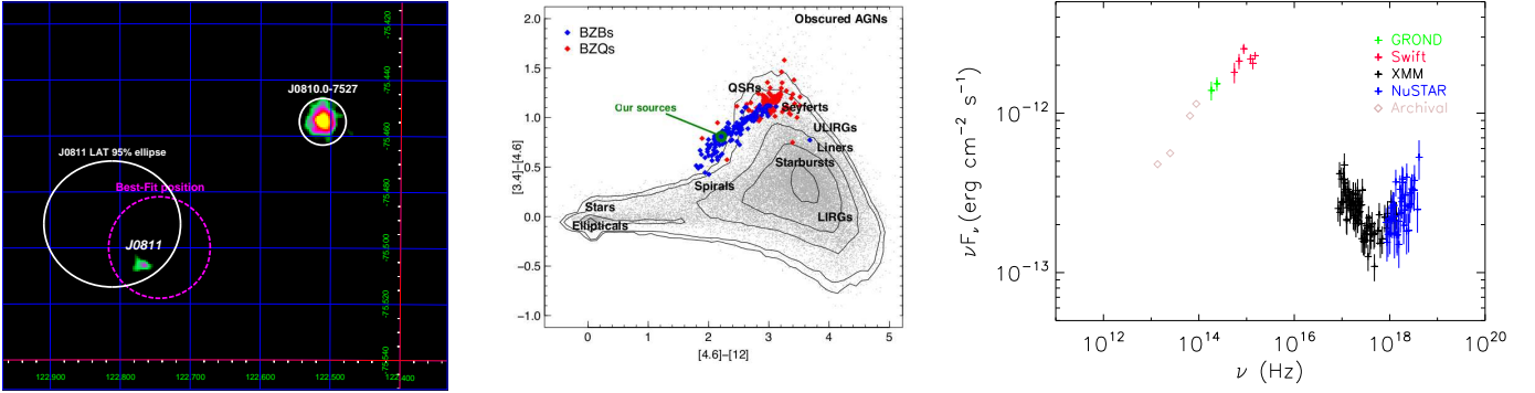
Figure 2. Left: NuSTAR image of the field containing J0811. The color scale is arbitrarily adjusted for better visibility. Fermi /LAT 3FGL ellipse (95%, white) and the best-fit circle (95%, magenta) are shown, and a R = 30'' circle is drawn around the serendipitous source (denoted as J0810.0-7527). Middle: Location of the sources we are studying in the WISE [3.4]-[4.6]-[12] \mu\text{m} color-color diagram (Figure taken from D’Abrusco et al. 2012). The four sources, including J0810, are located in the middle of the BZB (naming convention for BL Lac in the ROMA-BZCAT catalog) distribution. See D’Abrusco et al. (2012) for more detail. Right: Observed SED of the serendipitous source. Note that we used N_{\text{H}} = 6.9 \times 10^{20} \text{ cm}^{-2} , the optical extinction inferred value, for constructing the SED. Notice that this new source is quite hard, emitting more strongly in the NuSTAR band than in the XMM-Newton band.
