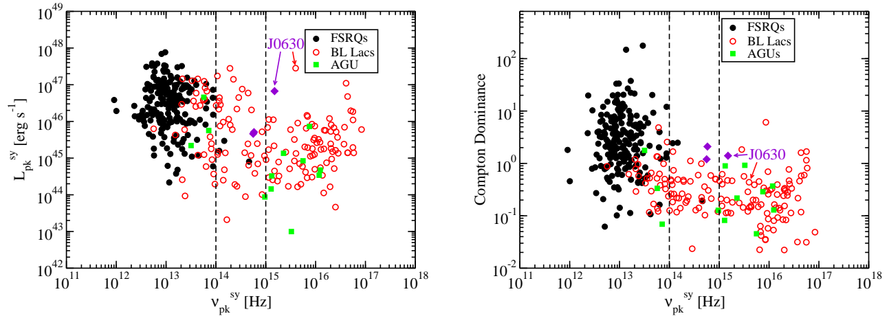
Figure 6. Left: Synchrotron peak luminosity vs. synchrotron peak frequency. Right: Compton dominance vs. synchrotron peak frequency. We use black filled circles for FSRQs, red empty circles for BL Lacs, and green squares for sources which are not clearly classified. The three BL Lacs we study are shown as purple diamonds. Note that the red circle for J0630 shows the position of the source reported in a previous study (Finke 2013).
