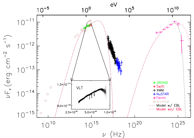
Figure 4. An SED model fit with (black dotted line) and without (red dotted line) the EBL absorption model (Finke ‘C’ in Table 4) for the J0630 data with a hard injection spectrum. The parameters for this model are: \delta_D = 73 , \theta_v = 0.74^\circ , B = 10 mG, R'_b = 2 \times 10^{14} cm, p_1 = 2.35 , \gamma_{\min} = 5 \times 10^3 , and \gamma_{\max} = 2 \times 10^5 .
