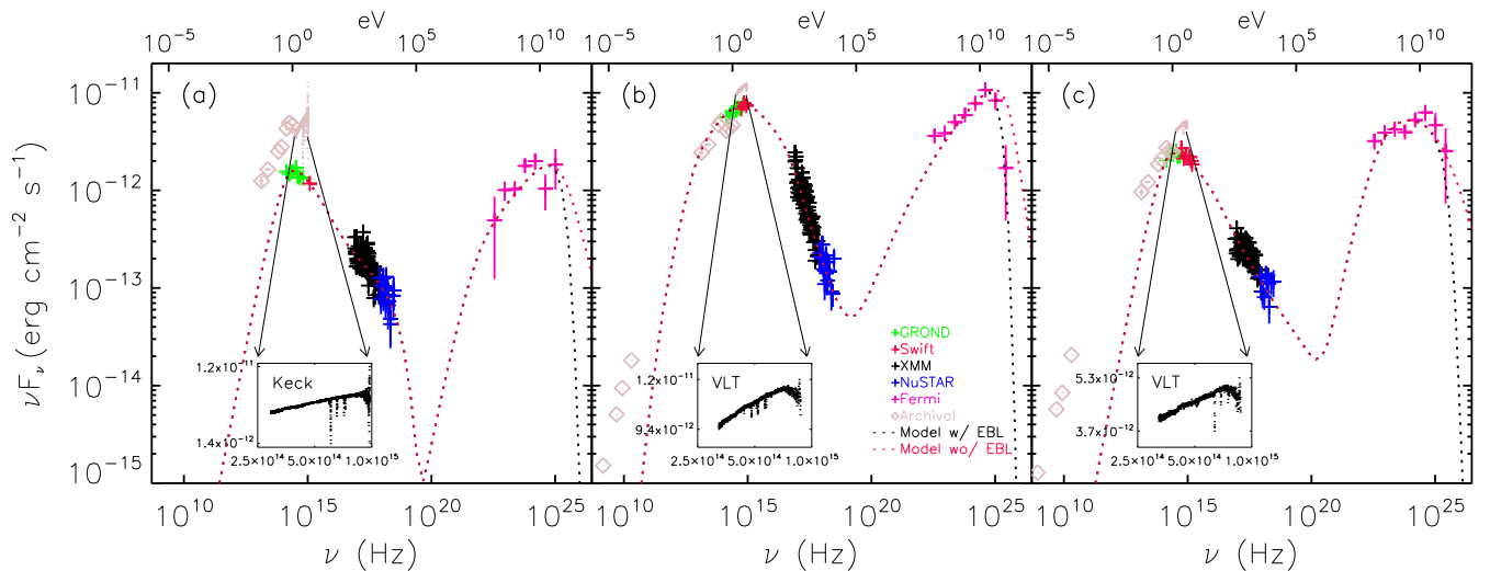
Figure 3. Observed broadband SED and best-fit models for (a) J0022, (b) J0630, and (c) J0811. Data points with an error bar are taken from the contemporaneous observations (Sections 2.1 and 2.2) and diamonds are from the archival observations (Section 2.3). The dashed lines are the best-fit SSC SED models of Boettcher et al. (1997) with (black) and without (red) EBL absorption (Finke et al. 2010). Note that the archival data are not taken contemporaneously even if they are plotted in the same color and symbol. The insets plot the VLT/Keck spectra of Shaw et al. (2013), showing the lack of emission lines and the low excitation absorption complexes placing lower limits on the redshift. These observations appear to have been in a brighter, harder optical state.
