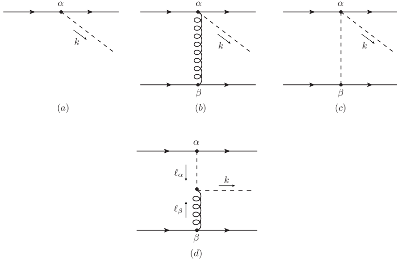
FIG. 3: Leading order Feynman diagrams in the perturbative expansion of the scalar emission amplitude \mathcal{A}_s(k) .
