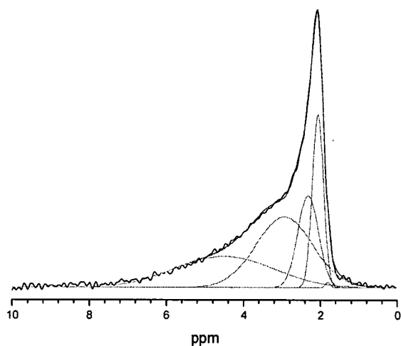
Figure 1S. ^1\text{H} MAS NMR spectrum of SSZ-33 after deboronation and dehydration at 250 °C.
