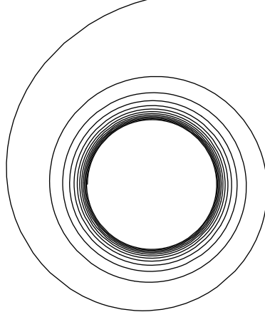
FIGURE 5. The limit cycle of a foliation.
